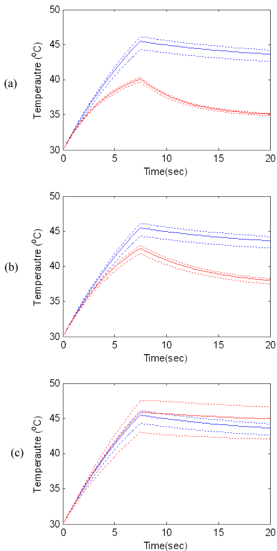
Figure 6: (a) Comparison of average temperatures (solid line) and maximum/minimum temperatures (dotted) time variation for Cell AP (blue) and Cell BP (red) with mid-size PHEV10 US06 driving scenario; (b) same for Cell AP (blue) and Cell CP (red); (c) same for Cell AP with different layer normal conductivity, 0.8 W/mK (blue) and 0.2 W/mK (red)
