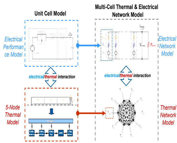
Figure 10: Example of an integrated thermal and electrical network model of a multi-cell battery
