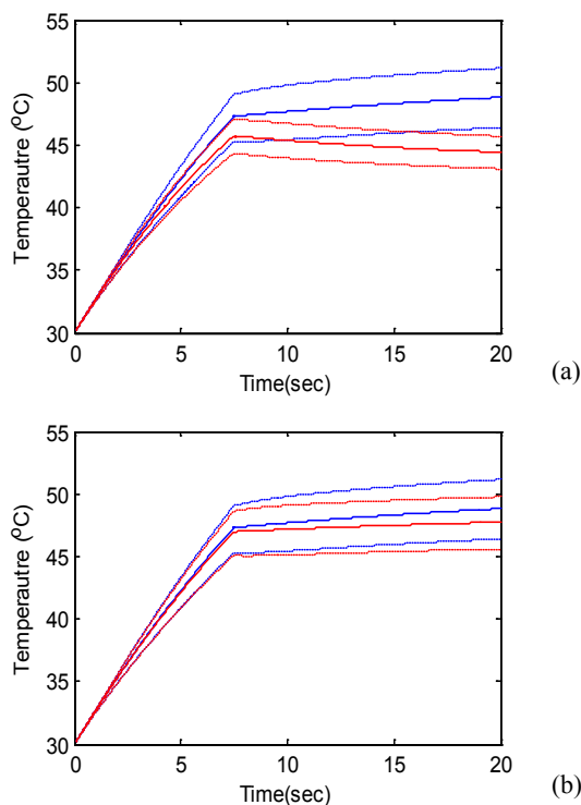
Figure 7: (a) Comparison of average temperatures (solid) and maximum/minimum temperatures (dotted) time variation for Cell AC (blue) and Cell BC (red) with mid-size PHEV10 US06 driving scenario; (b) same for Cell AC (blue) and Cell CC (red)
