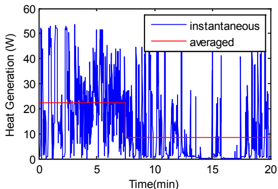
Figure 5: Instantaneous and averaged heat generation rate per cell (20 Ah)
