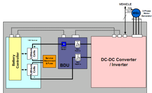
Figure 3: Electrical components of a battery pack, from [3]
