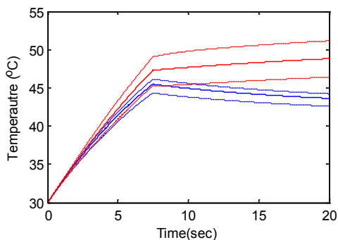
Figure 8: Comparison of average temperatures (solid) and maximum/minimum temperatures (dotted) time variation for Cell AP (blue) and Cell AC (red) with mid-size PHEV10 US06 driving scenario
