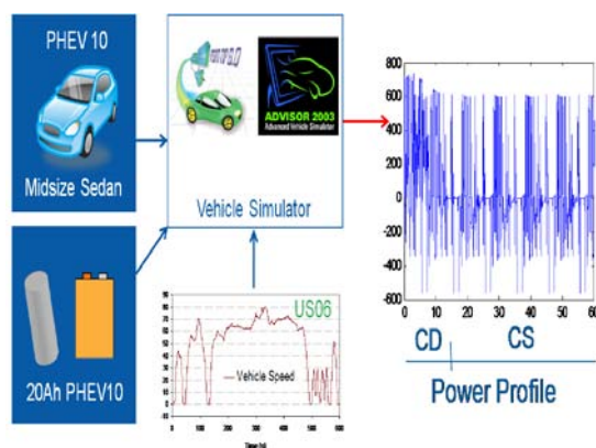
Figure 4: Schematics for 20 Ah cell power profile evaluation with PHEV10 application (120 Wh/kg cell, 78 BSF)
