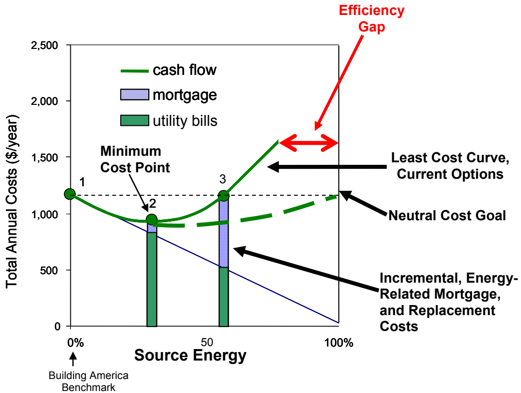
Figure B-1. Example Cost/Performance Curve
