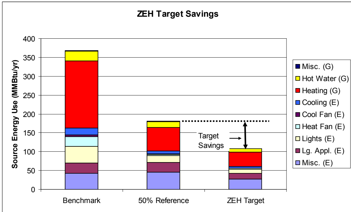
Figure C-5. Cold Climate Region (Chicago), Gas Space Heating
