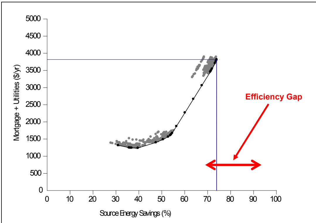
Figure B-3. Marine Climate Region (Seattle), Electric Space Heating
