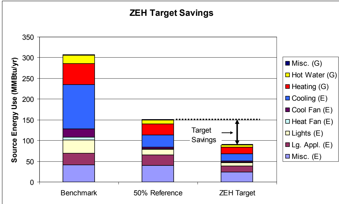
Figure C-2. Hot Humid Climate Region (Houston), Gas Space Heating
