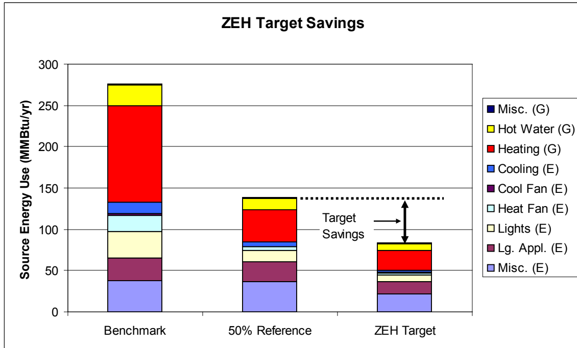
Figure C-1. Northern Marine Climate Region (Seattle), Gas Space Heating
