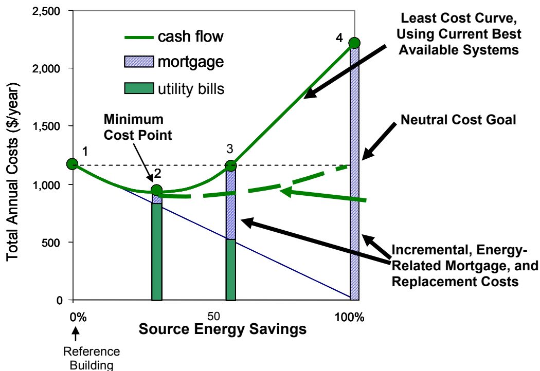
Figure 1. ZEH Whole-House Cost/Performance Target
