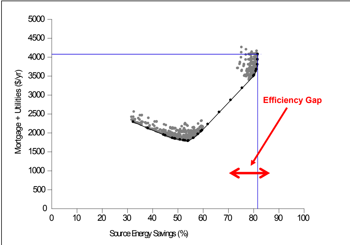
Figure B-4. Hot Humid Climate Region (Houston), Gas Space Heating
