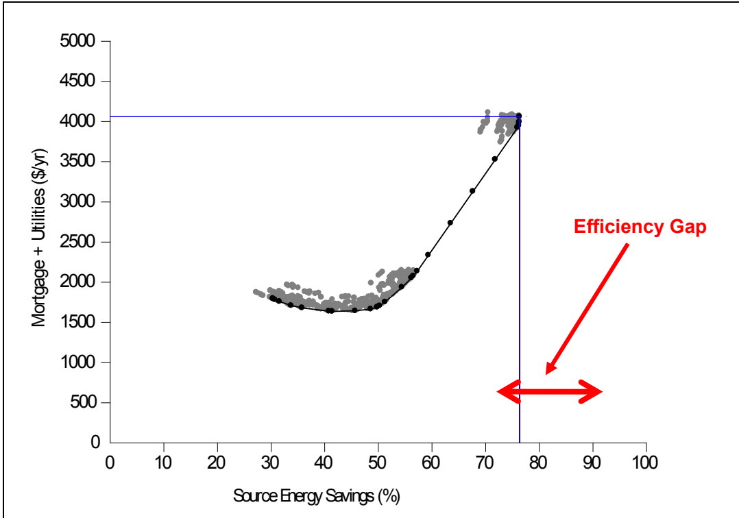
Figure B-2. Marine Climate Region (Seattle), Gas Space Heating
