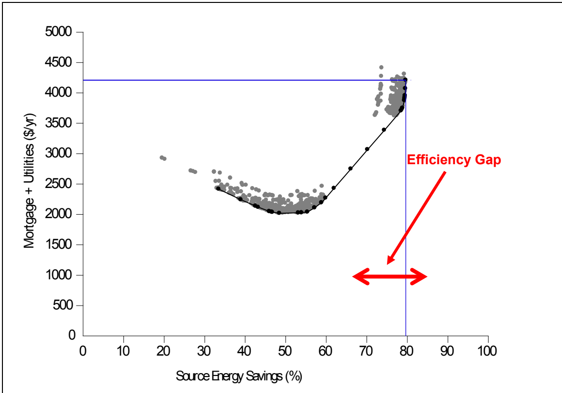
Figure B-5. Hot Humid Climate Region (Houston), Electric Space Heating
