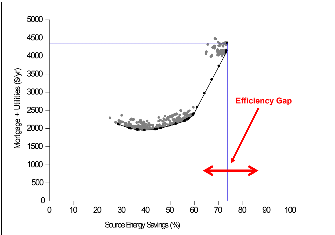
Figure B-11. Cold Climate Region (Chicago), Electric Space Heating
