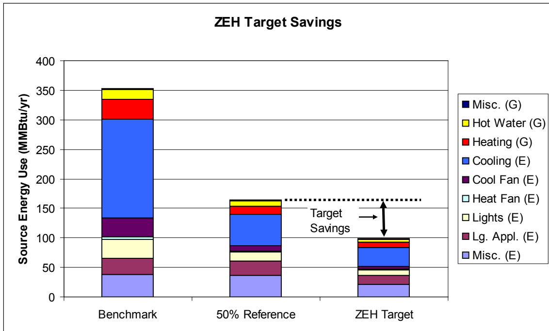
Figure C-3. Hot/Mixed Dry Climate Region (Phoenix), Gas Space Heating
