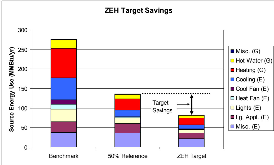
Figure C-4. Mixed Humid Climate Region (Atlanta), Gas Space Heating
