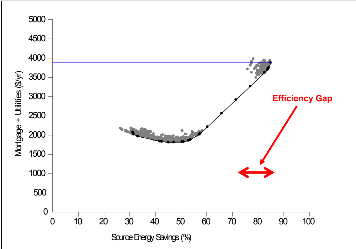
Figure B-8. Mixed Humid Climate Region (Atlanta), Gas Space Heating
