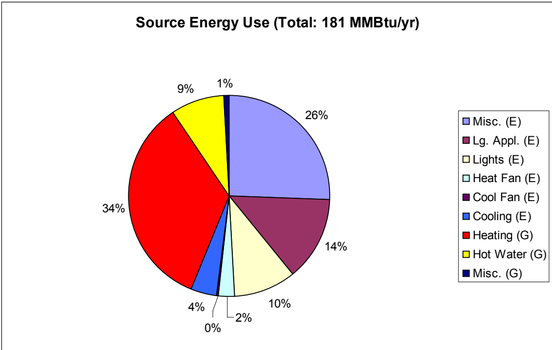
Figure D-5. Cold Climate Region (Chicago), Gas Space Heating
