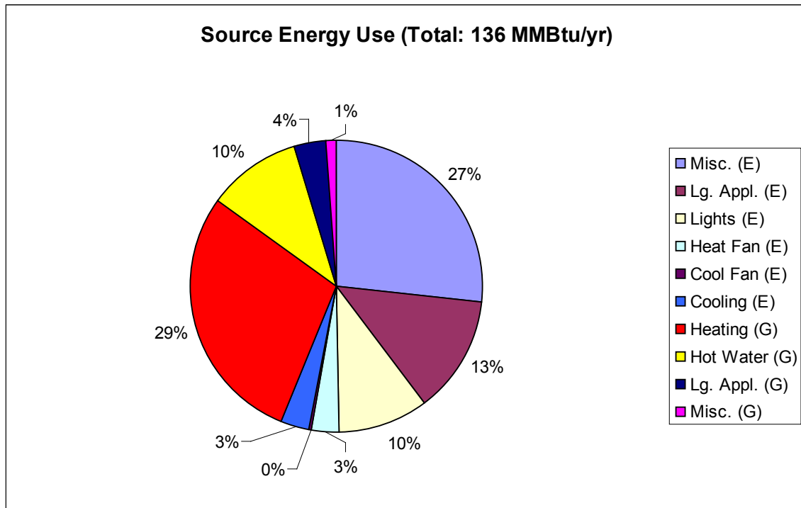
Figure D-1. Marine Climate Region (Seattle), Gas Space Heating
