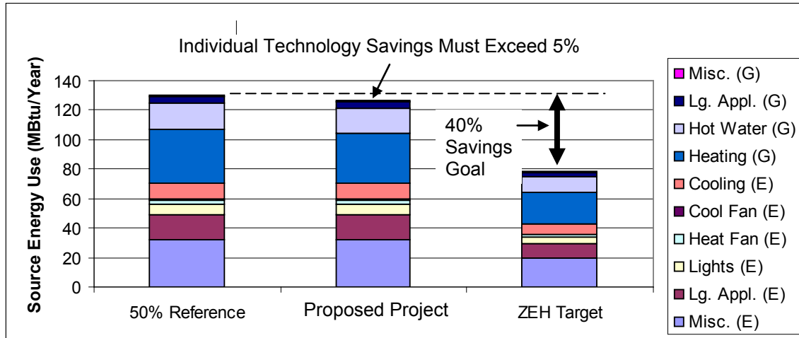
Figure 9. Minimum Energy Savings Requirement for ZEH Technologies Projects
