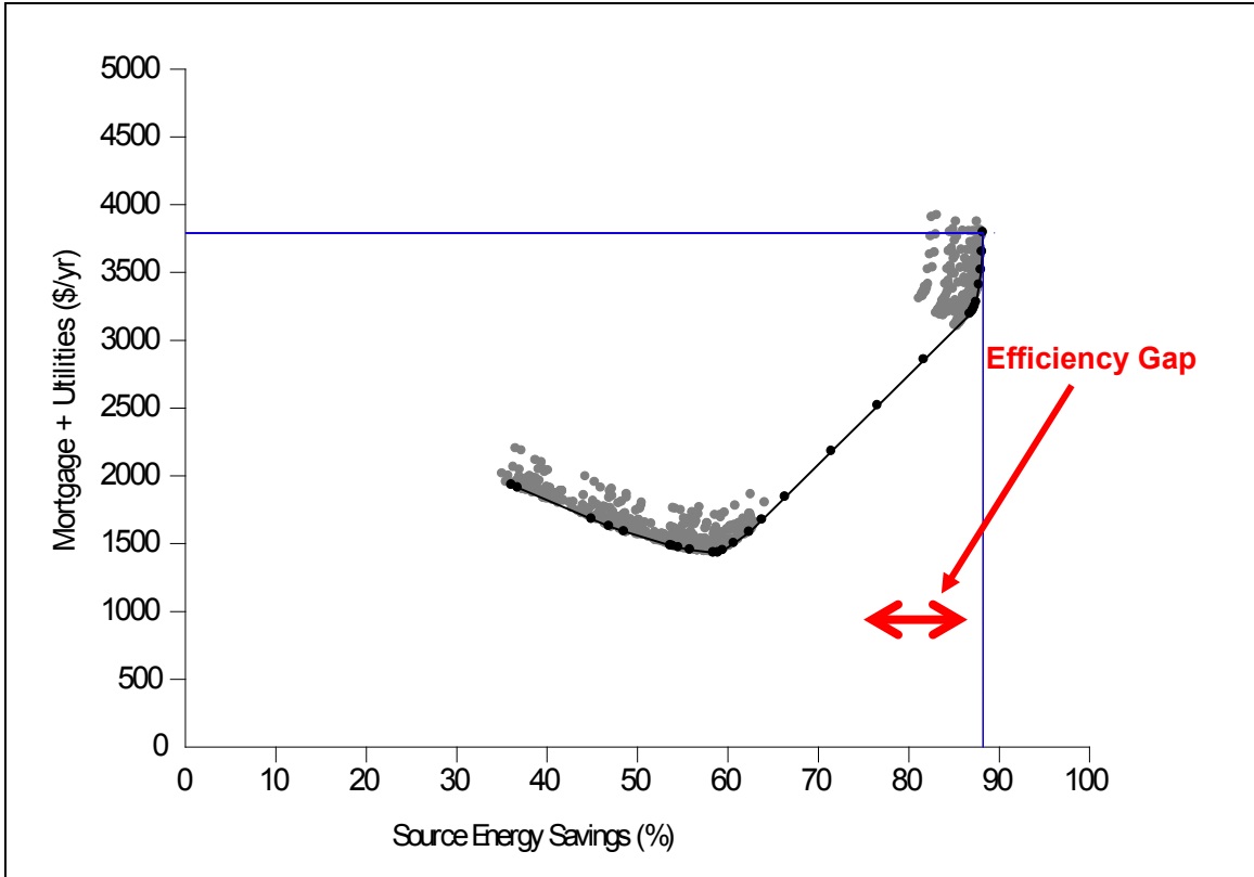
Figure B-6. Hot/Mixed Dry Climate Region (Phoenix), Gas Space Heating
