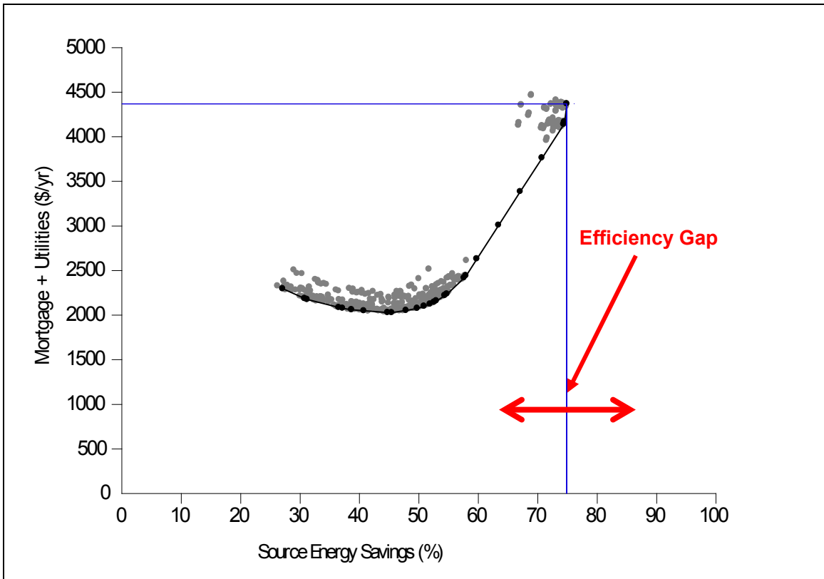
Figure B-10. Cold Climate Region (Chicago), Gas Space Heating
