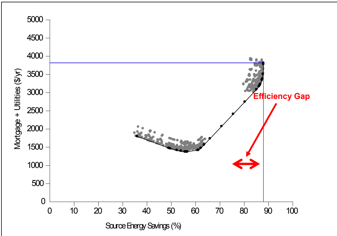
Figure B-7. Hot/Mixed Dry Climate Region (Phoenix), Electric Space Heating
