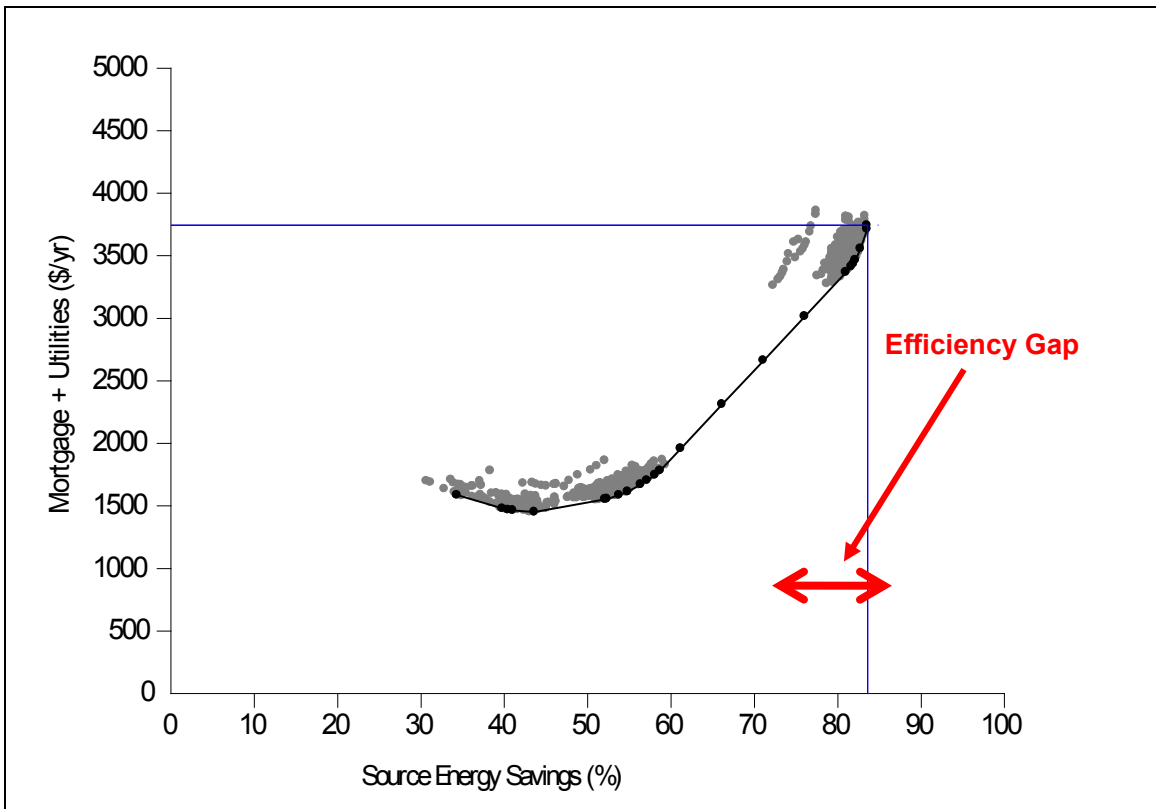
Figure B-9. Mixed Humid Climate Region (Atlanta), Electric Space Heating
