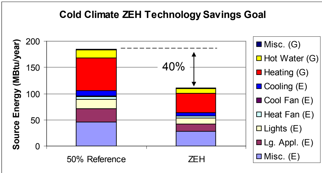
Figure 8. Energy Savings to Be Provided by an Expanded ZEH Technology Research Program (see Appendix C for a summary of energy saving opportunities in other climates)
