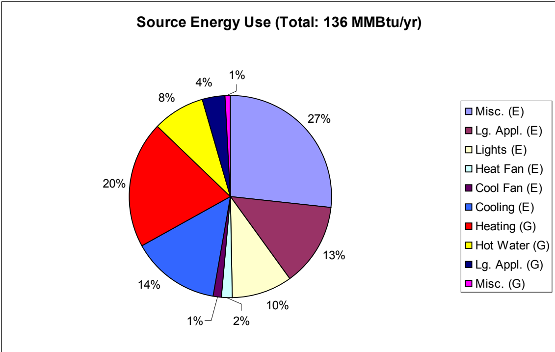
Figure D-4. Mixed Humid Climate Region (Atlanta), Gas Space Heating
