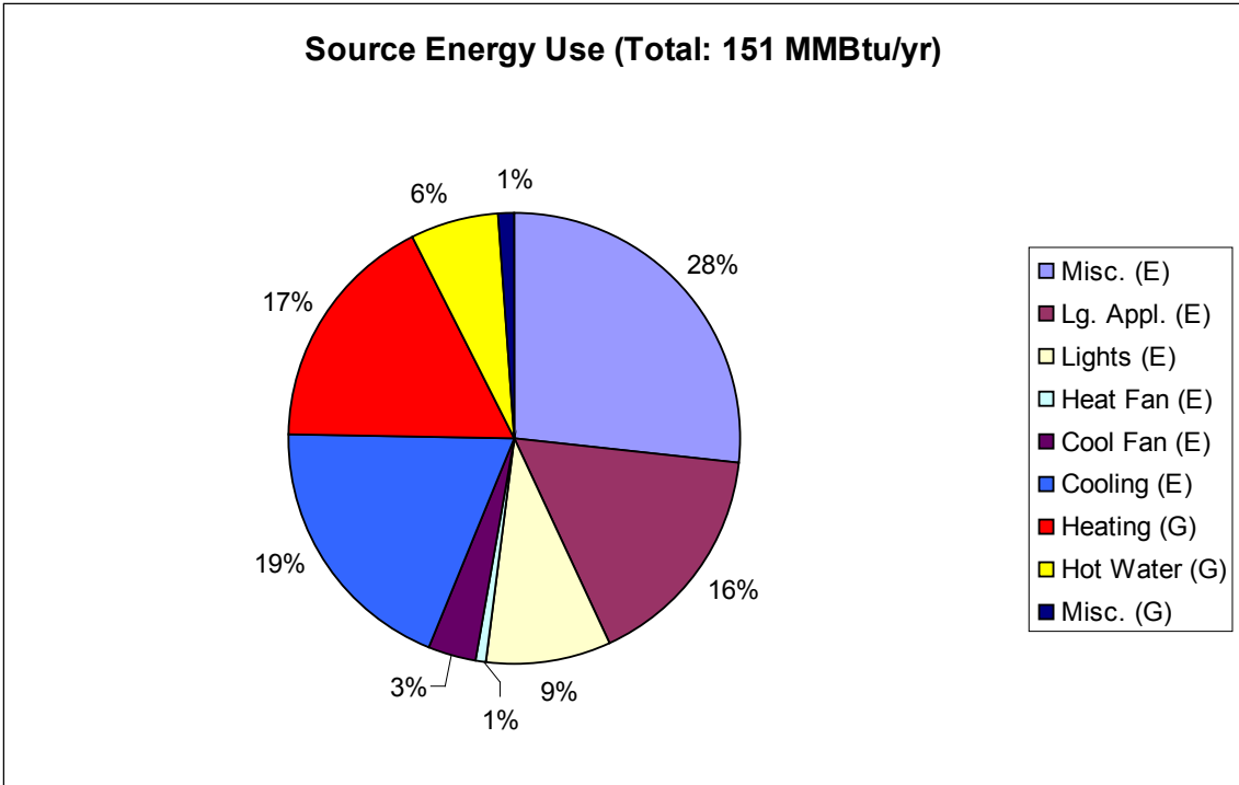
Figure D-2. Hot Humid Climate Region (Houston), Gas Space Heating
