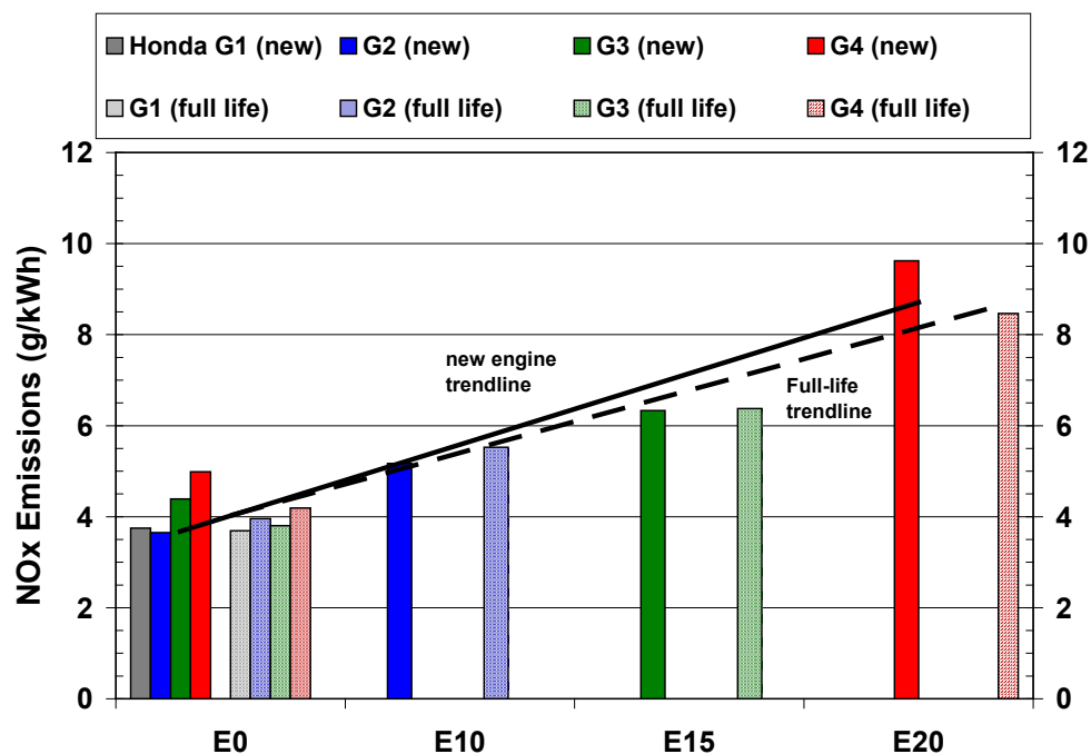
Fig. D.10. Nitrogen oxide ( \text{NO}_x ) emissions for Class I Honda generator engines at new and full-useful-life (full-life) condition. Solid colors represent tests in the new condition while striped bars of the same color represent the same engine at the full-life condition.
