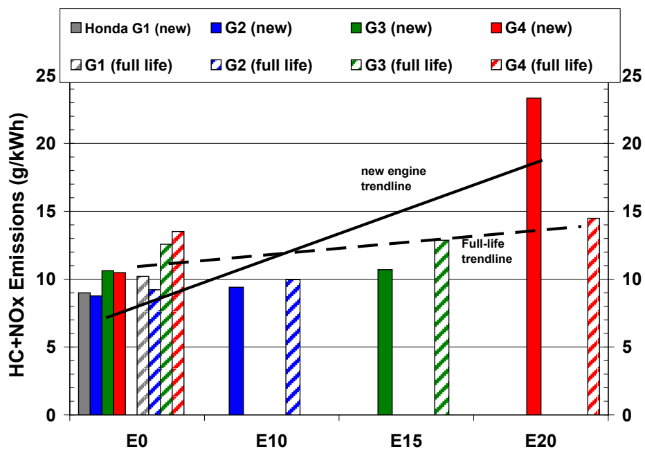
Fig. D.11. Hydrocarbon (HC) + nitrogen oxide ( \text{NO}_x ) emissions for Class I Honda generator engines at new and full-useful-life (full-life) condition. Solid colors represent tests in the new condition while striped bars of the same color represent the same engine at the full-life condition.
