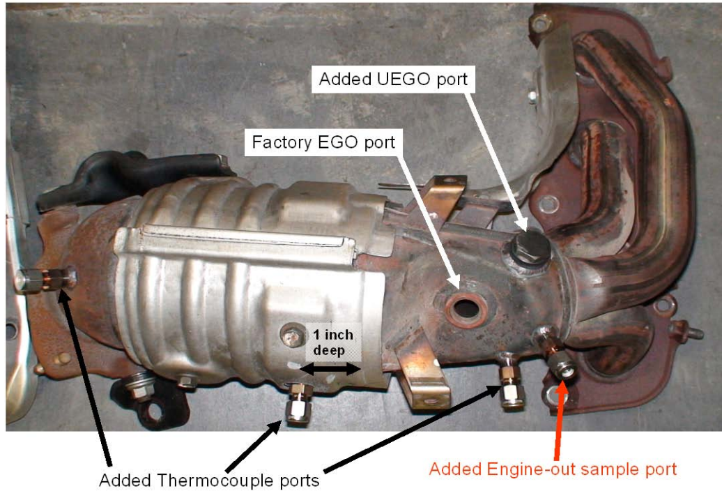
Fig. A.1. Example of vehicle exhaust system instrumentation, including universal exhaust gas oxygen sensor (UEGO) and temperature and exhaust gas sample ports.
