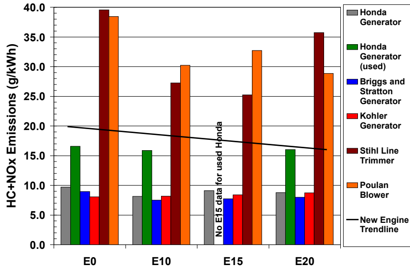
Fig. 3.13. Hydrocarbon (HC) + nitrogen oxide (NO x ) emissions for pilot study engines. Decreasing NO x and increasing HC temper any drastic changes in HC + NO x . Trendline for average of all five new engines shows overall decrease with increasing ethanol.
