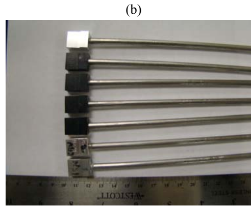
Figure 2: Illustration of the principle behind self-oscillating jets, (a) cross-sectional view of fluidic nozzle, (b) different nozzles tested.
