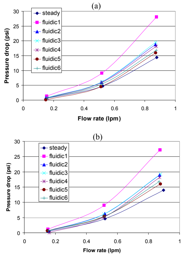
Figure 6: Pressure drop as a function of flow rate with 1.1 mm target distance, (a) free-surface, (b) submerged.
