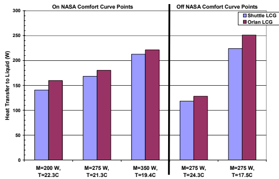
Figure 9: Heat Transfer to LCG Fluid
