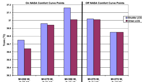
Figure 8 Core Temperatures
