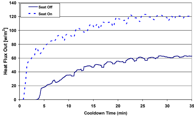
Figure 5 Heat Loss from ADAM’s Back and Bottom
