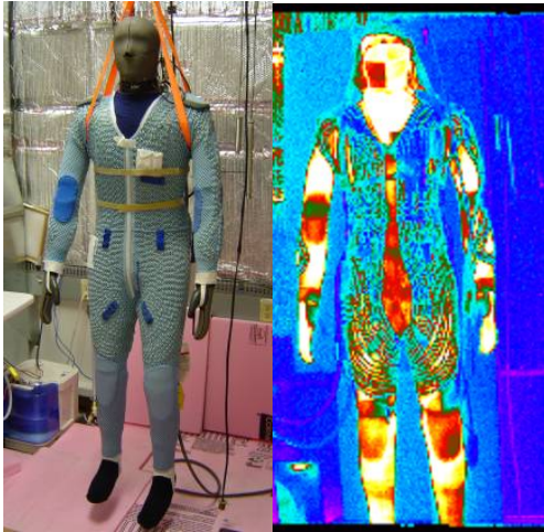
Figure 4. ADAM in the Orlan LCG
