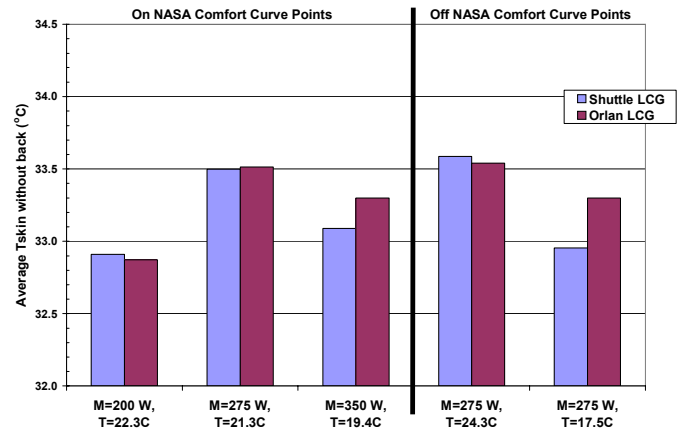
Figure 7. Average skin temperature without the back for Shuttle and Orlan LCGs
