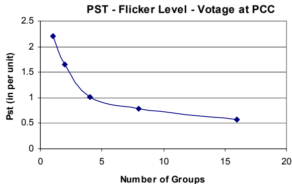
Fig. 9. Pst level of the voltage at the PCC as a function of the number of the groups in the wind farm.
