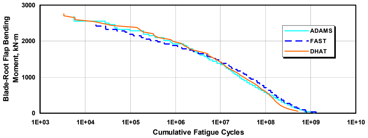
Figure 11. WP 1.5 blade-root flap bending moment cumulative spectra.
