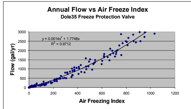
Fig. 6. Correlation between annual flow of consumed water (y) and the Air Freezing Index (x).
