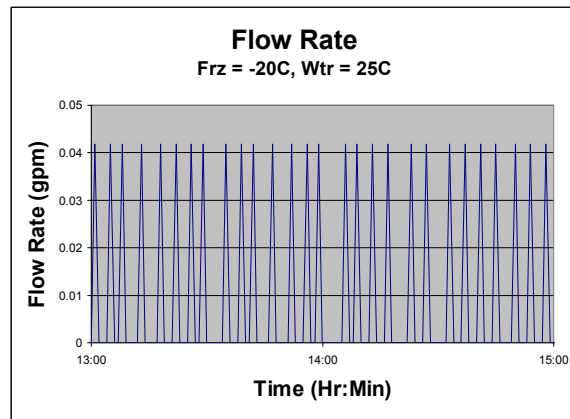
Fig. 5. Flow rate versus time for the Eaton/Dole FP35 valve. Data were stored in one minute intervals. The valve cycled on about every four minutes, although cycles can be missed due to flow meter pulse resolution.
