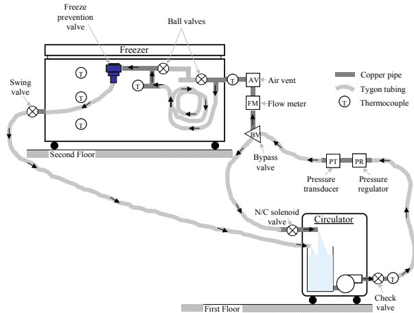
Fig. 4: Schematic diagram of the FPV experiment.
