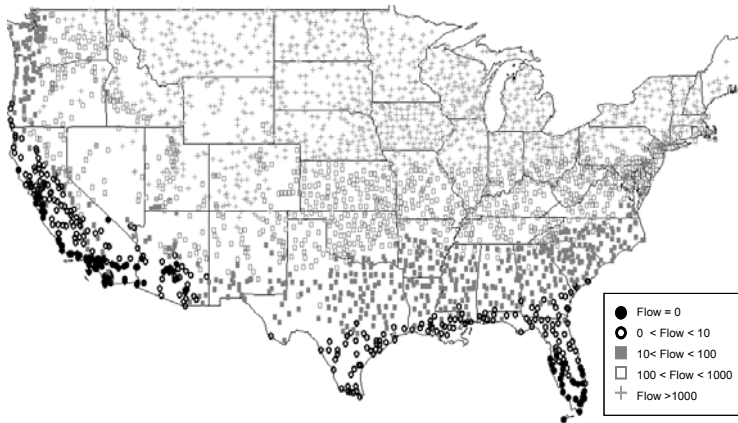
Fig. 8: Flow (gallons/year) through an Eaton/Dole FP-35 pipe freeze prevention valve. This valve would be chosen for freeze-protection of piping in the attic. The 1000 gal/yr border might be a reasonable cutoff for use of FPV.
