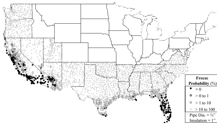
Fig. 9: Probability of at least one freeze in 20 years, for mild climate states, 3/4" pipe with 1" insulation. The dark dots indicate regions where it would be safe to install passive systems with insulated pipes in the attic. The region is quite small, and corresponds to where passive ICS are installed today. The region could be extended by using FPVs for pipe freeze protection, although reliability concerns demand multi-levelled, fail-safe protection for such a critical function.
