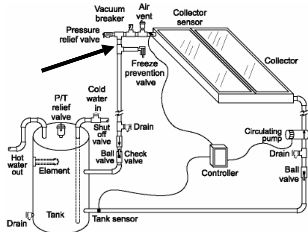
Fig. 1. A direct circulation system schematic. The freeze prevention valve (FPV) is shown near the collector outlet.
