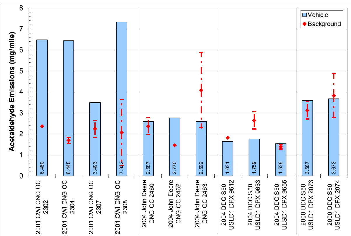
Figure 18: Acetaldehyde Emissions
