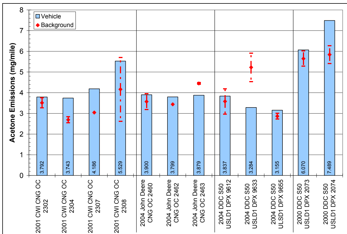
Figure 19: Acetone Emissions
