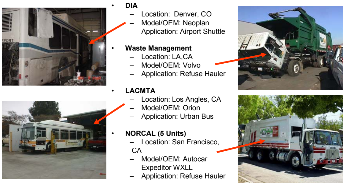
Figure 10: Field Test Vehicles
