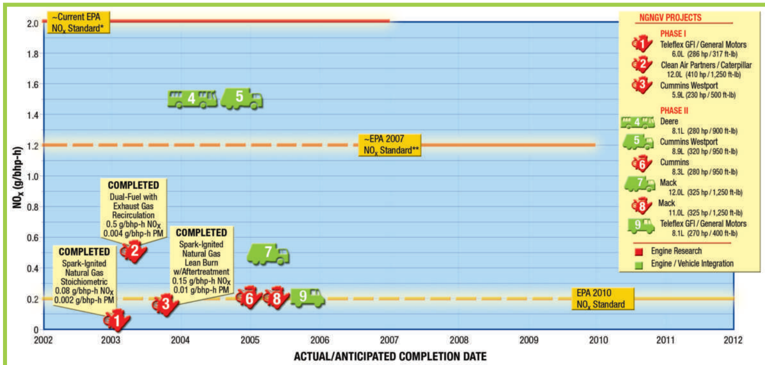
Figure 1. Results and Goals for NGNGV Engine and Vehicle Projects
