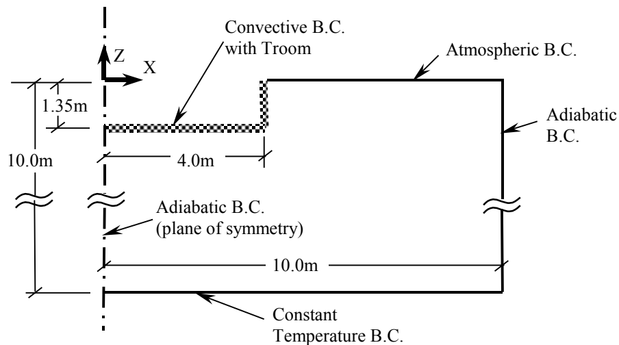
Figure 2. Two-dimensional view of the computation domain and boundary conditions for the IEA BESTEST case 990
