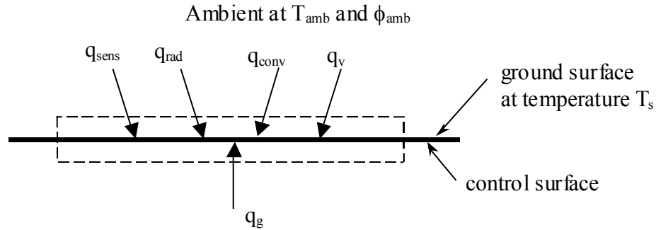
Figure 1. Thermal energy balance at the ground surface
