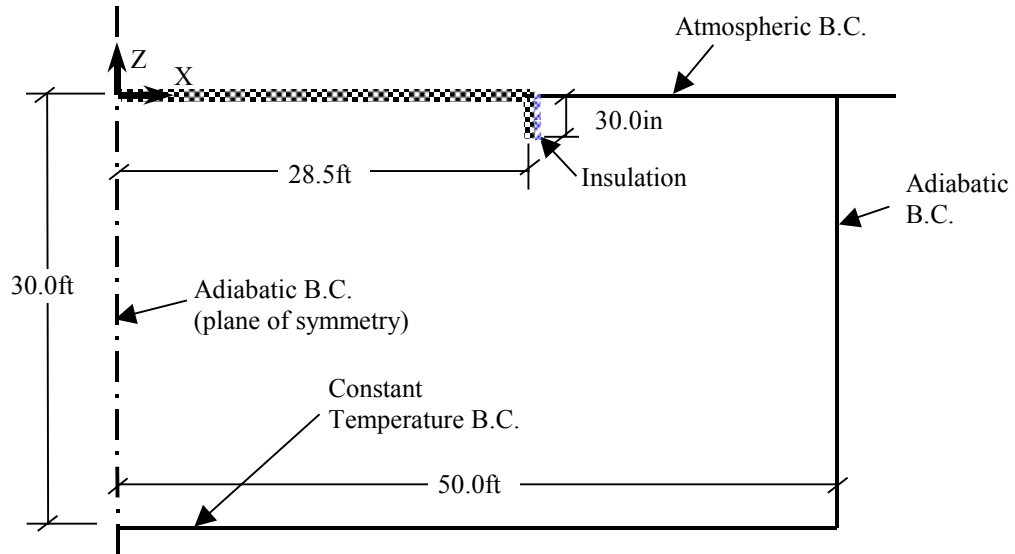
Figure 3. Two-dimensional view of the computation domain and boundary conditions for the HERS BESTEST cases L302BC and L304BC
