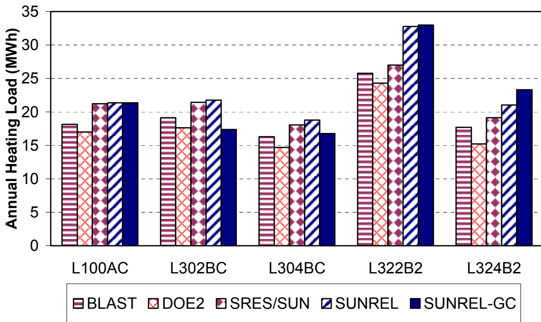
Figure 6. Annual heating loads for the HERS base case and the ground-coupled cases
