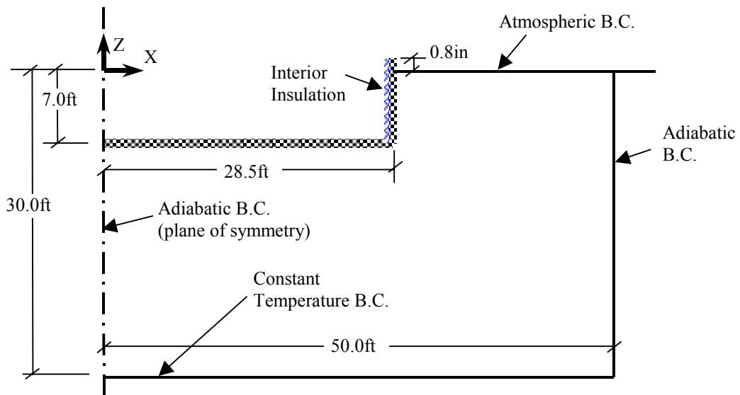
Figure 4. Two-dimensional view of the computation domain and boundary conditions for the HERS BESTEST cases L322B2 and L324B2
