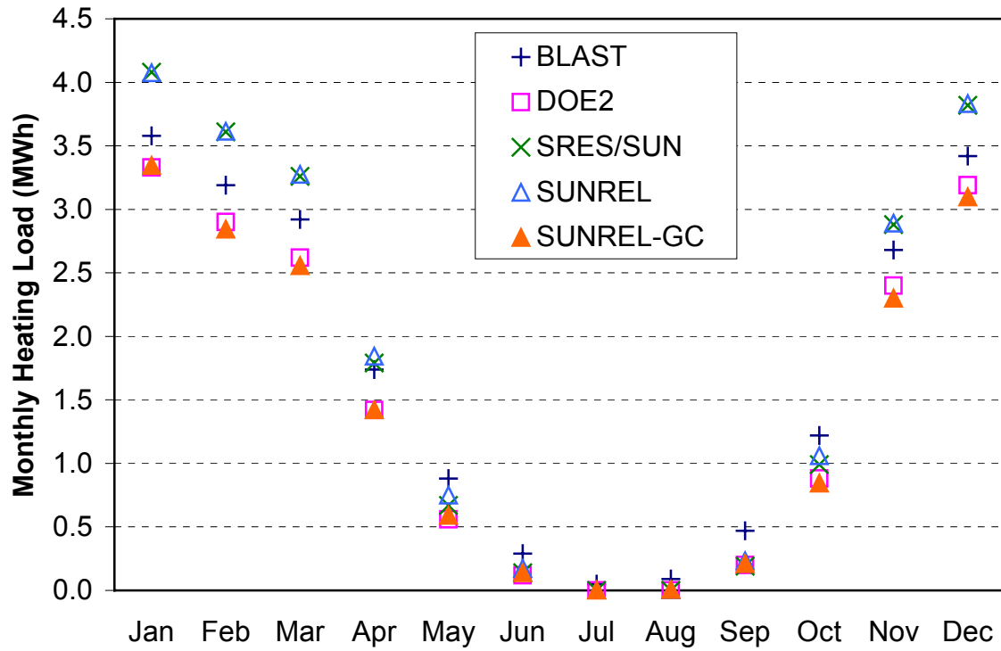
Figure 7. Monthly heating loads for the uninsulated slab-on-grade case L302BC
