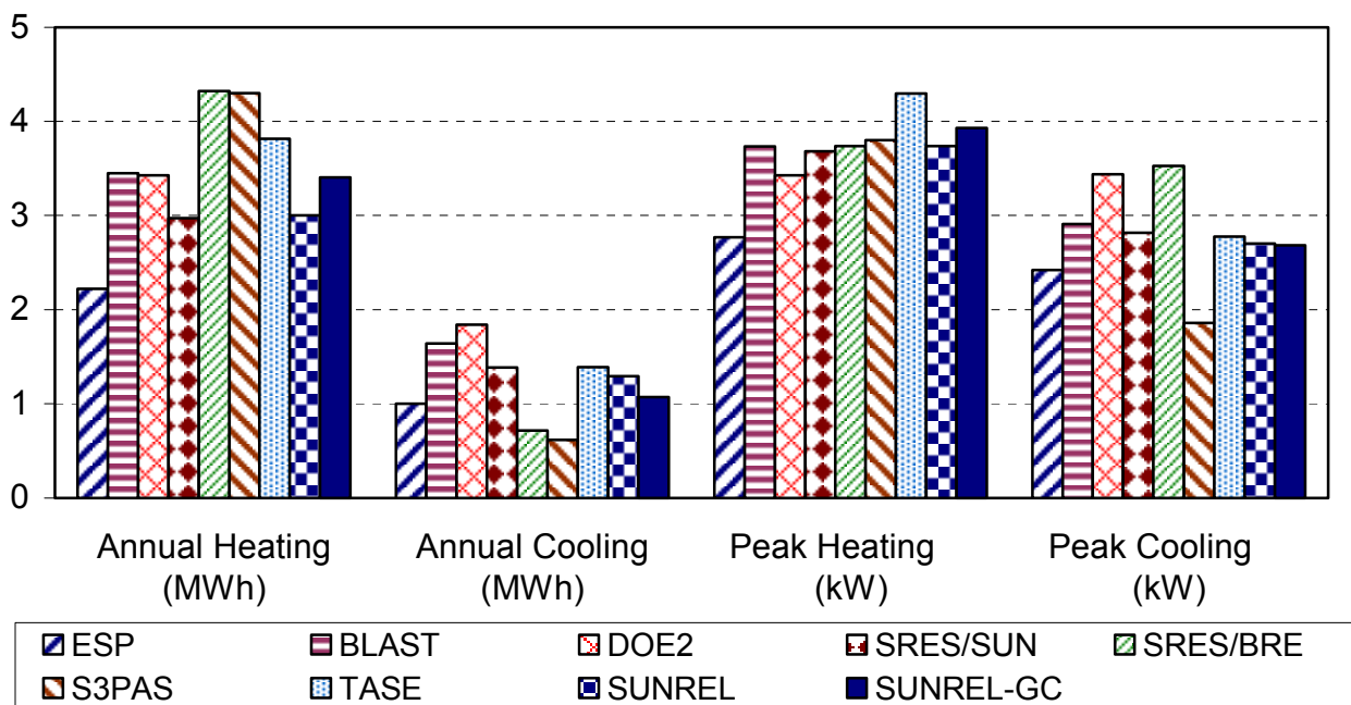
Figure 5. Annual heating and cooling energy and peak hourly heating and cooling loads for the uninsulated basement of the IEA case 990
