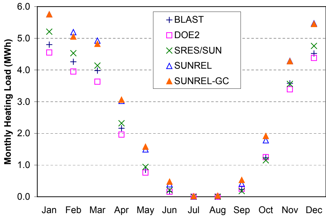
Figure 8. Monthly heating loads for the uninsulated basement case L322B2
