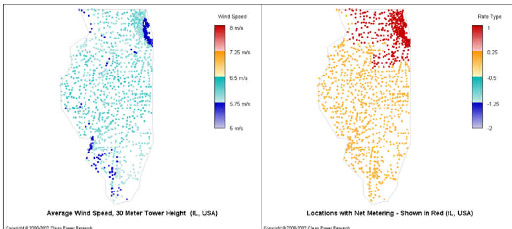
FIGURE 4. AVERAGE ANNUAL WIND SPEED AT 30 METERS.
