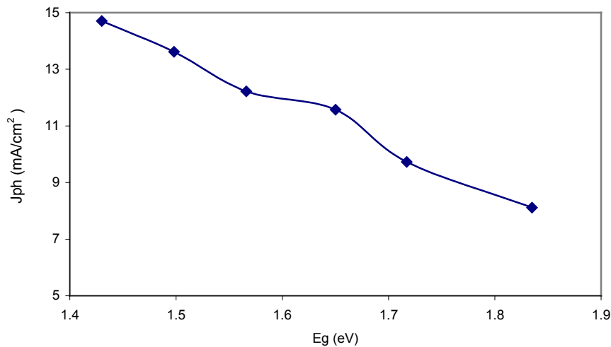
Figure 3-15. Current integrated from QE for a-SiGe cells, deposited on bare SS, with different bandgaps.
