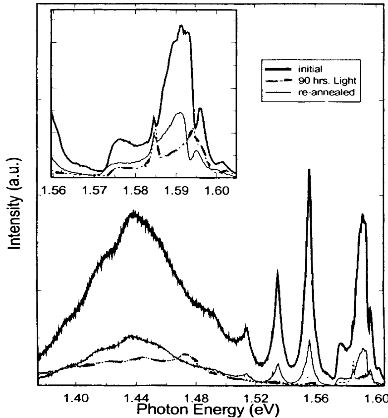
Fig. 2-5. PL of CdTe:Cu immediately after diffusion, after 90 hr light exposure, and after re-anneal.
