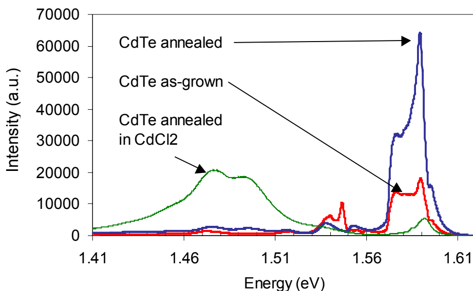
Figure 2-12: Photoluminescence from CdTe single crystals as-grown, annealed at 387 C, and annealed at 387 C in CdCl 2 .
