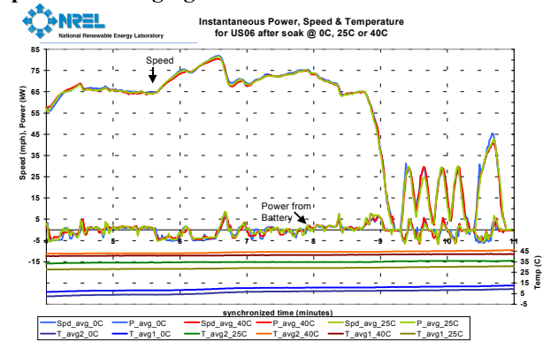
Plot 4: 180–600 seconds from US06 warm-up cycle at 0°C, 25°C, and 40°C
