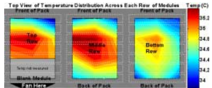
Figure 6: US06 at 25°C before the fan kicks on for cooling
