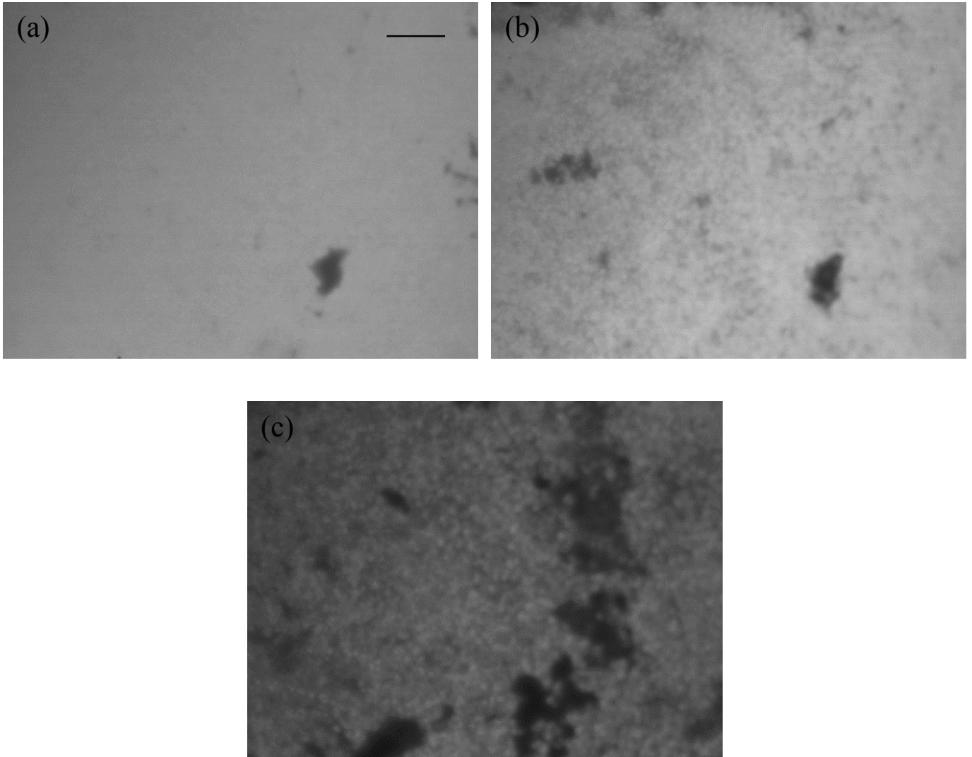
Fig 9. Front-wall LBIC images of a cell with Cu/HgTe/graphite back-contact prepared with First Solar CdTe/CdS samples following (a) 0, (b) 18 and (c) 35 hours treatment at 200°C in air in the dark. Bar = 100 \mu\text{m} .
