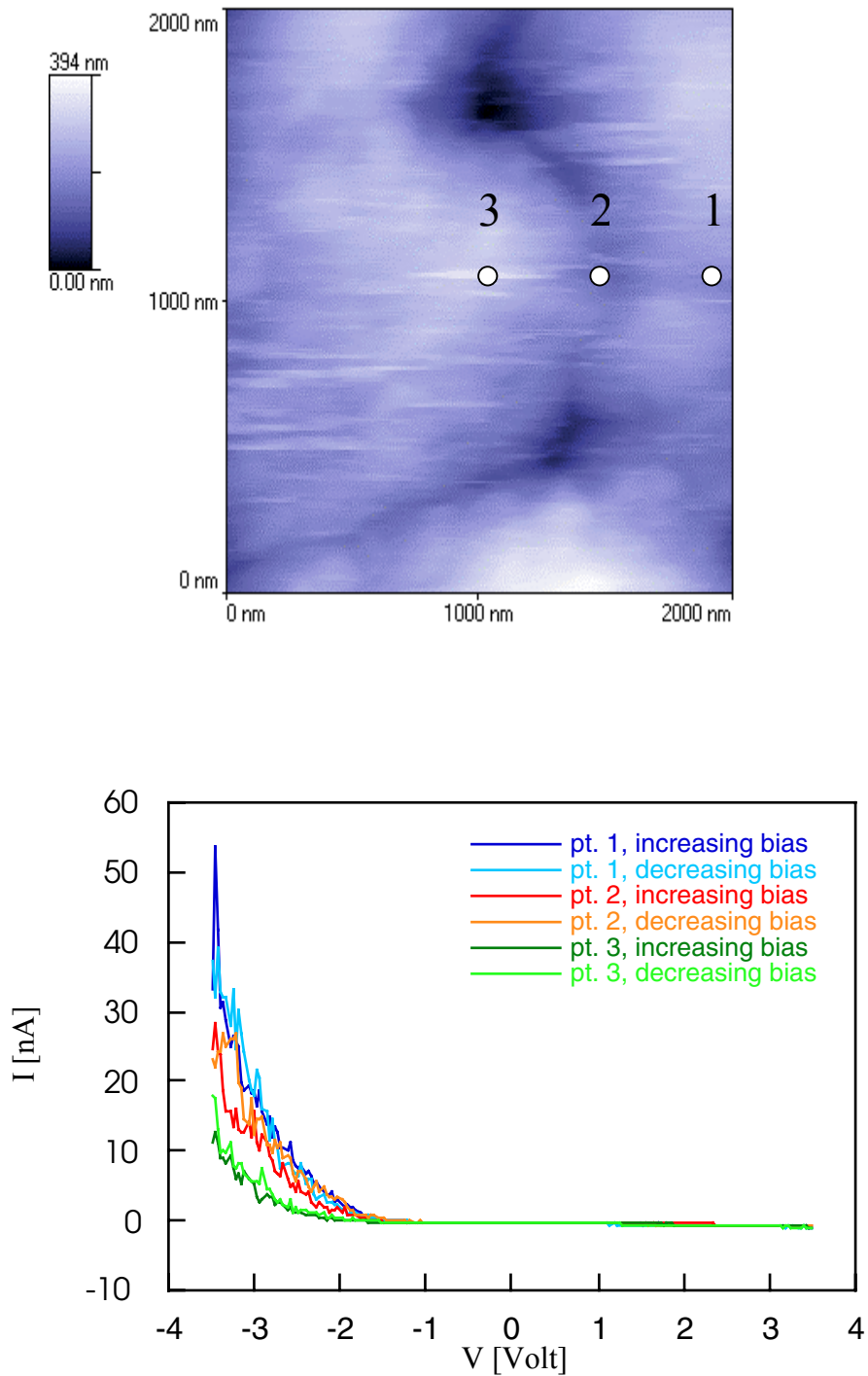
Fig. A1 Spatially resolved IV measurements of CdTe film, using a conductive AFM tip: top. Locations of the tip (the counter-contact is the SnO 2 substrate), bottom. IV spectroscopy in the respective locations
