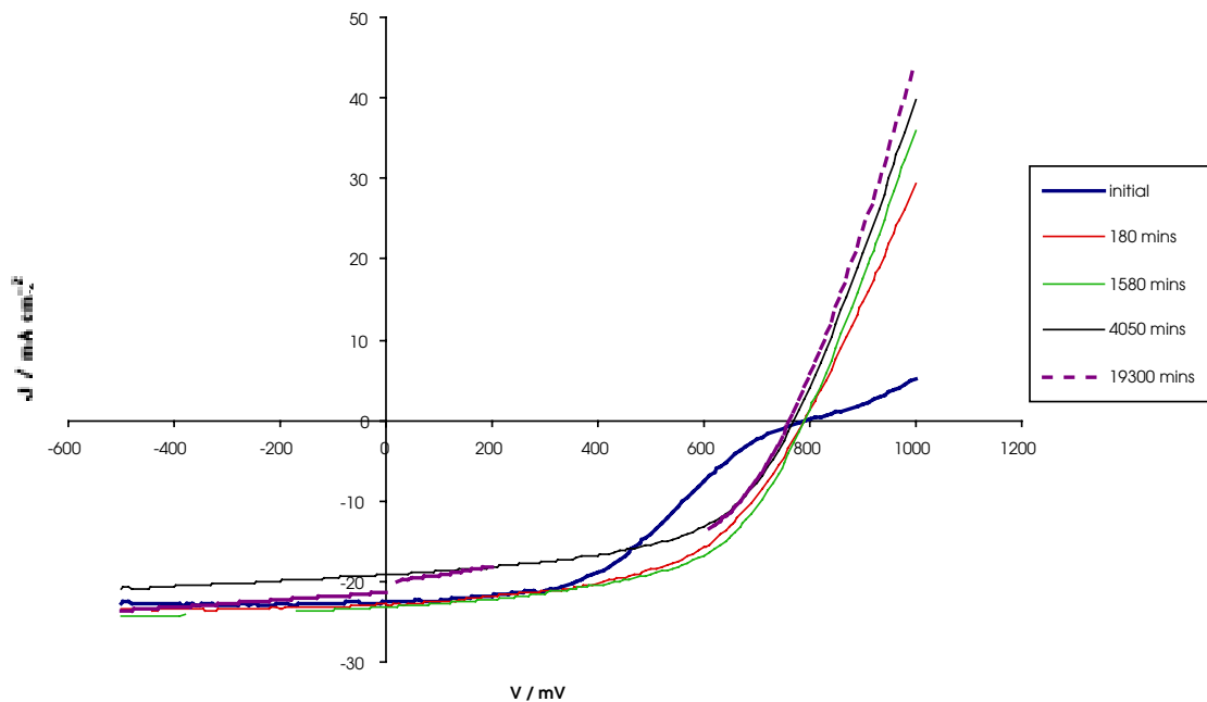
Fig. 8. Light I-V plots of CdS/CdTe solar cell with Cu/HgTe/graphite back contact prepared with USF sample recorded following 200 °C treatment over time. Prior to treatment cell parameters were: efficiency 7.6% , fill factor 42% , V_{oc} \sim 800 mV and J_{sc} -23 mA cm -2 . At the conclusion of the experiment cell parameters were 7%, 50%, 740 mV and -18 mA cm -2 , respectively.
