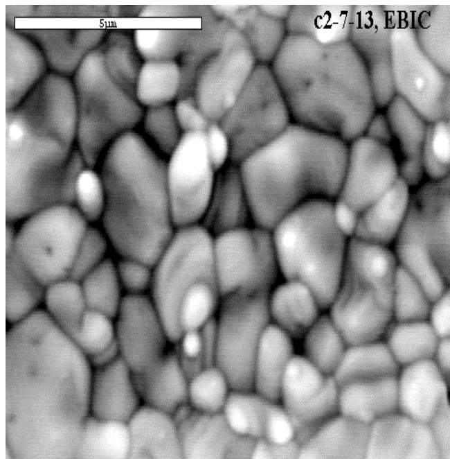
Fig. A4 CdTe film surface SEM micrographs: a. topography, b. EBIC
