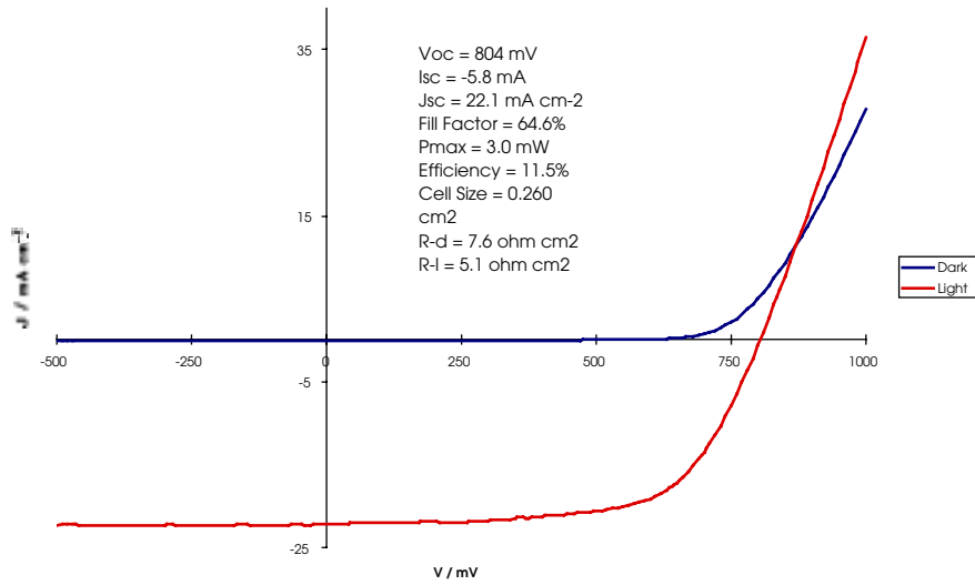
Fig. 5 Light and dark I-V plots of CdS/CdTe solar cell with Cu/HgTe/graphite back contact prepared on First Solar sample. A typical cell has a V_{oc} \sim 800 \text{ mV} , J_{sc} \sim 21\text{-}22 \text{ mA cm}^{-2} , fill factor of 60-65% and series resistance (under illumination) of 4-6 \Omega \text{ cm}^2 . Cells of 11.5% showed improved J_{sc} ( >26 \text{ mA cm}^{-2} ) or fill factor ( \sim 65\% ).
