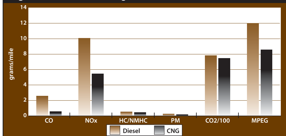
Figure 16. Emissions testing results for UPS CNG and diesel trucks
