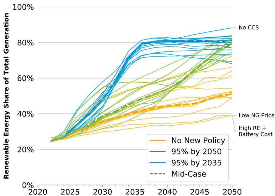
Figure 7. Renewable energy share over time across the Standard Scenarios. Renewable energy share is defined as annual renewable energy generation divided by total generation.
