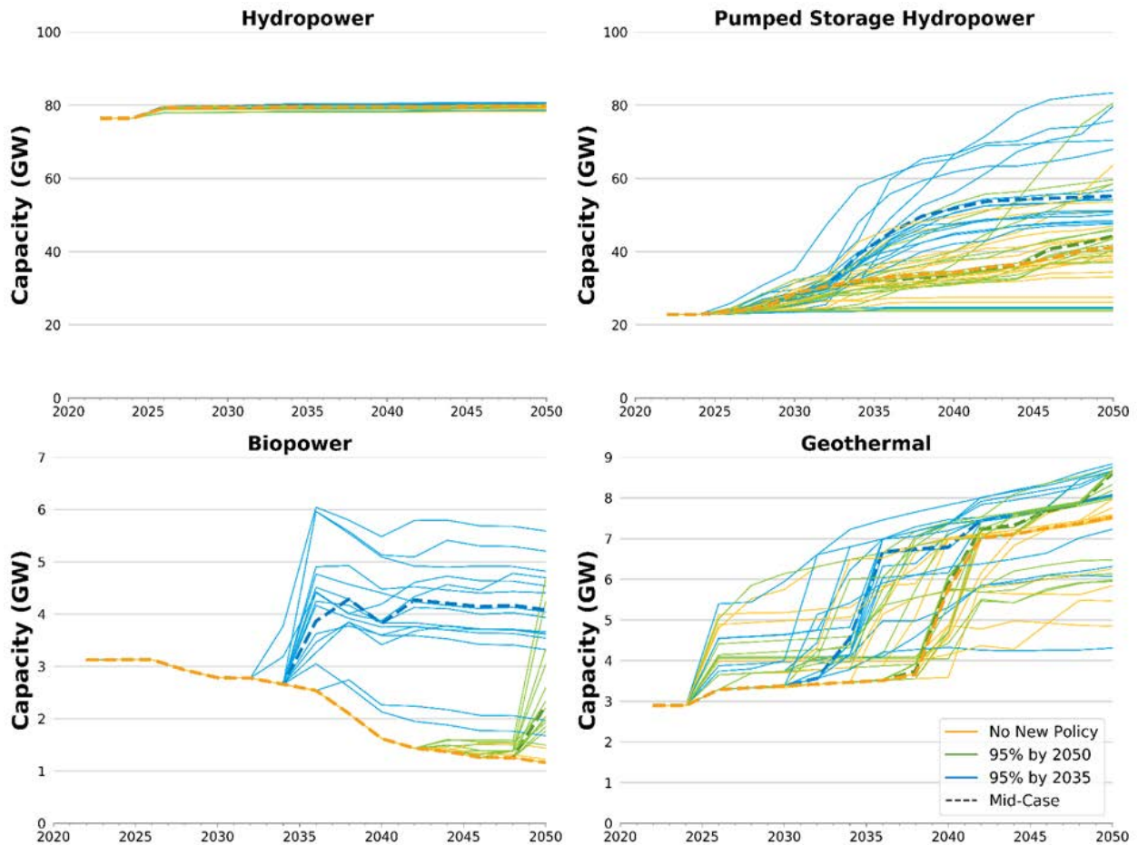
Figure A-5. Capacity by fuel type for the other RE technologies across the Standard Scenarios. The dashed line is the Mid-case scenario. Note that the scale is different in the charts. Biopower capacity includes capacity fitted with CCS.
