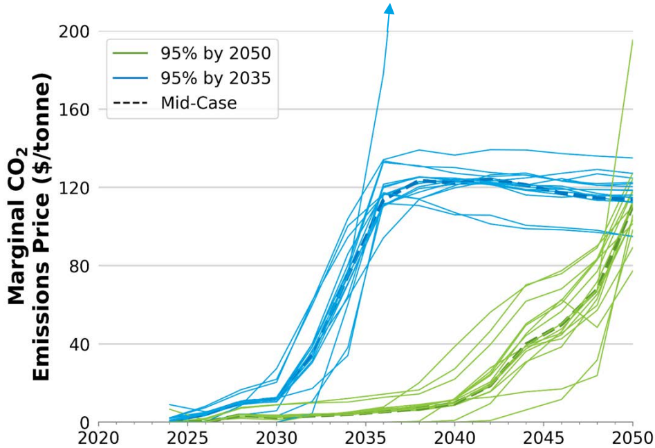
Figure 16. Marginal CO 2 emissions cost from the carbon emission limit. This value is the shadow price from the CO 2 cap imposed in the model. The scenarios that go above $150/tonne are those that do not allow CCS technologies to be built.
