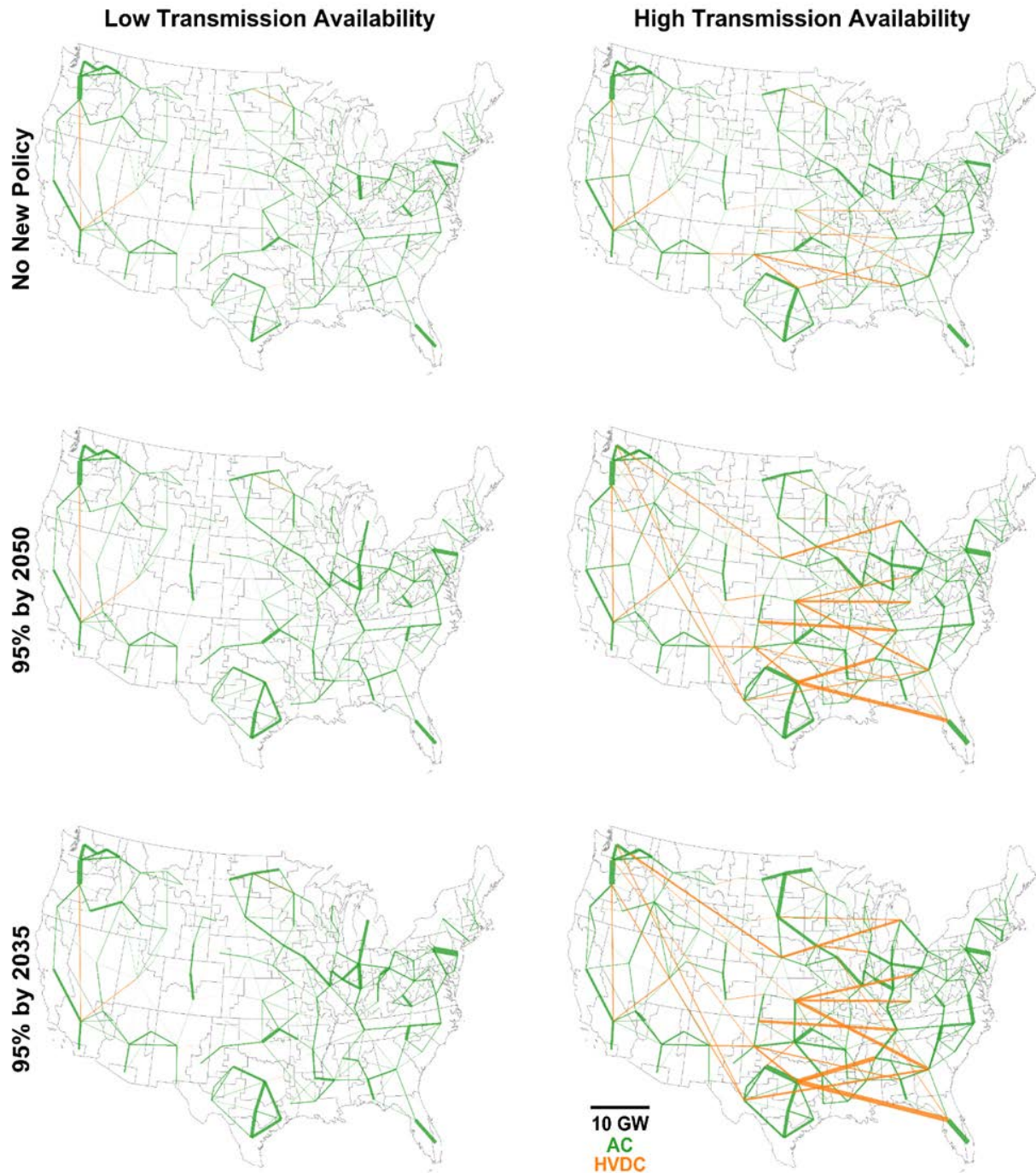
Figure 9. Total inter-regional transmission capacity in 2050 for the scenarios indicated. AC is alternating current and HVDC is high-voltage direct current.
