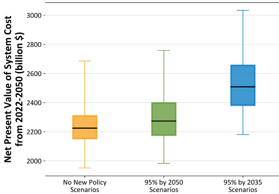
Figure 14. Net present value of system costs for the Standard Scenarios using a box-and-whiskers plot. The boxes show the 25 th -75 th percentile of results, the black bar is the median value, and the whiskers show the full range of results. System costs are the net present value (2020$) of the U.S. bulk power system from 2022 through 2050 using a 5% real discount rate. The Mid-case with No New Policy has a system cost of $2,225 billion dollars.
