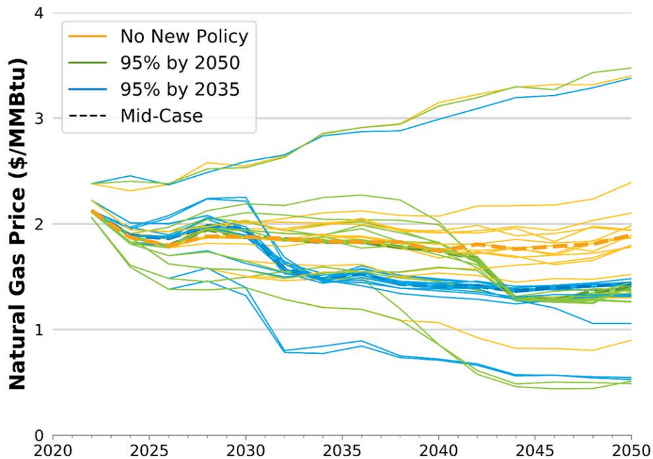
Figure A-2. Natural gas price outputs from the suite of ReEDS scenarios.
