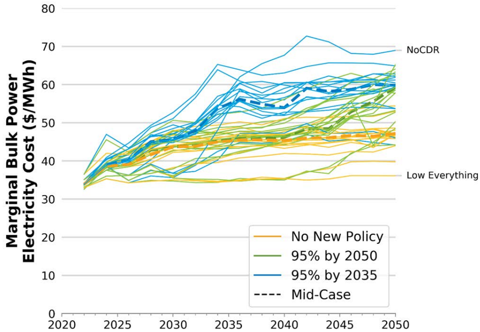
Figure 15. Marginal bulk power electricity cost over time across the Standard Scenarios. This bulk power cost does not include any distribution or administration costs, and it is calculated using the marginal costs from Figure 12.
