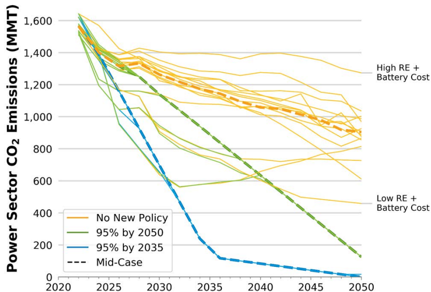
Figure 10. Power sector emissions over time across the Standard Scenarios. The highest and lowest emissions scenarios in 2050 are labeled, along with the low retirement scenario and the Low RE Cost scenario. The Mid-case scenario is the dashed line. MMT is million metric tonnes.
