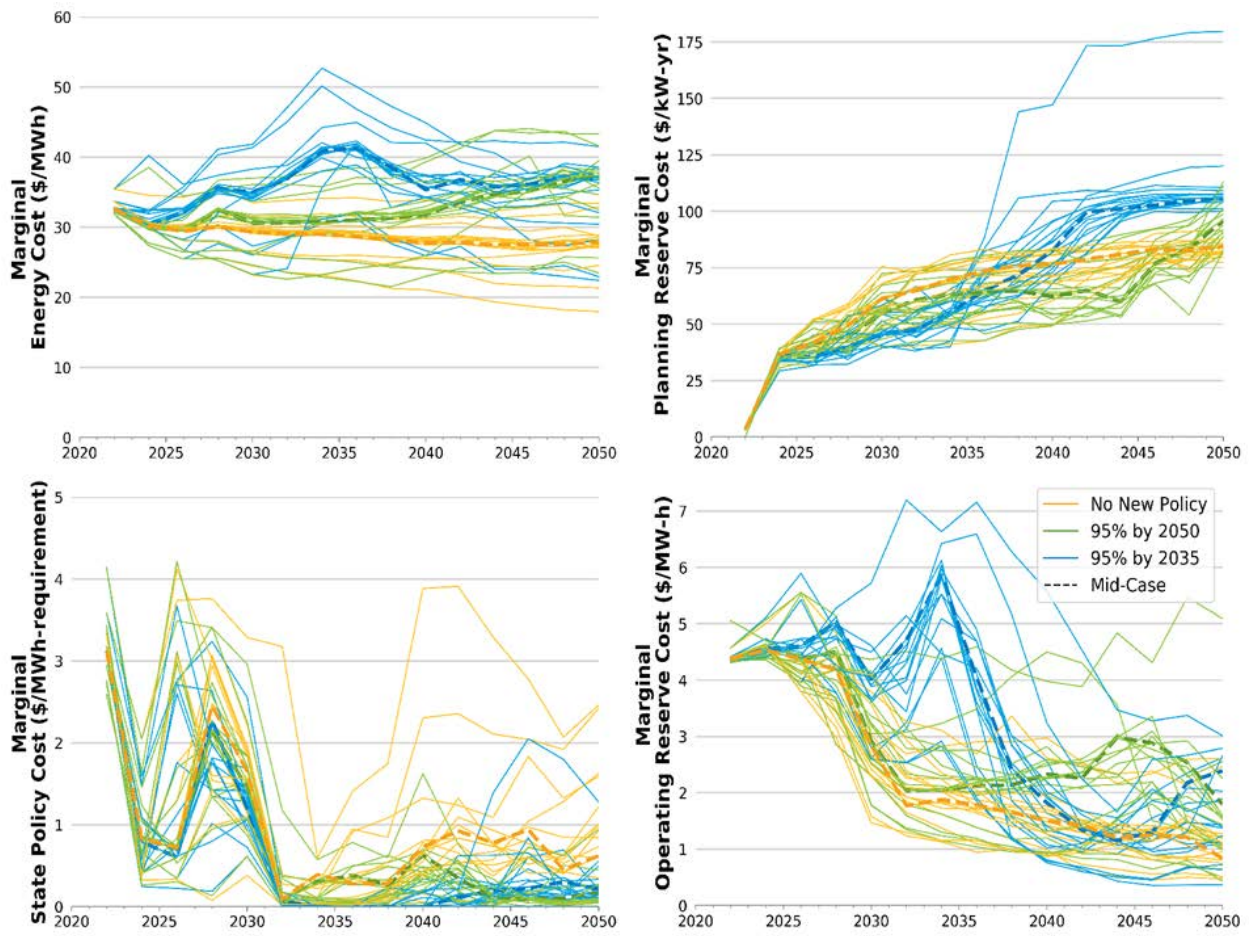
Figure 12. National annual average marginal costs for the services indicated across the Standard Scenarios. The dashed line shows the Mid-case for the three emission reduction trajectories. The marginal operating reserve cost is the sum of the three operating reserve products: regulation, spinning, and flexibility. The outlier in the top right plot is the No CCS scenario. Note that the units and scales are different in each plot.
