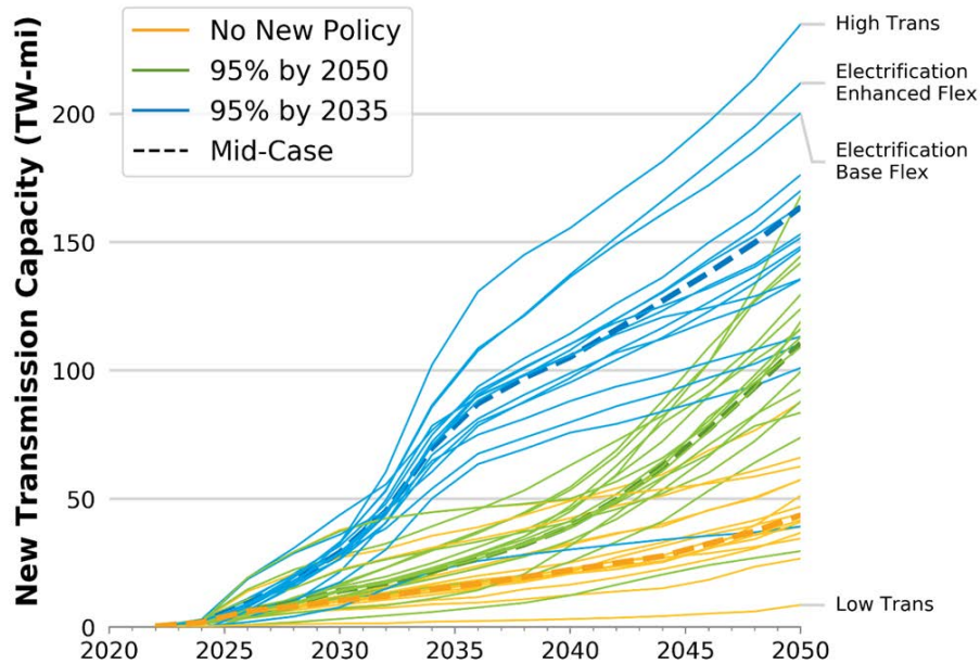
Figure 8. New long-distance transmission capacity over the Standard Scenarios. This reported capacity does not include the capacity of spur lines for connecting wind and solar plants to the transmission system. For reference, the scenarios start with 148 TW-mi in 2020.
