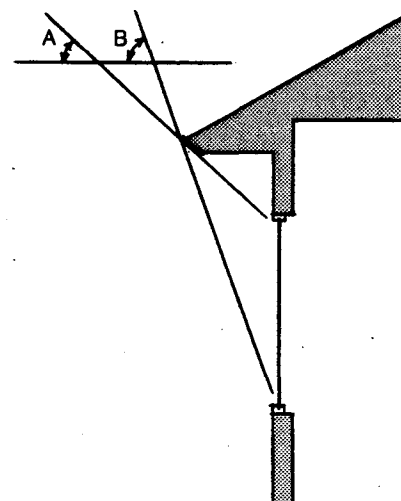
South Overhang Sizing In Rapid City, an ideally sized south overhang should allow full exposure of the window when the sun has a noon altitude of 27 degrees (angle A) and fully shade the window when the sun has a noon altitude of 64 degrees (angle B).
