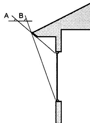
South Overhang Sizing In Tulsa, an ideally sized south overhang should allow full exposure of the window when the sun has a noon altitude of 35 degrees (angle A) and fully shade the window when the sun has a noon altitude of 72 degrees (angle B).
