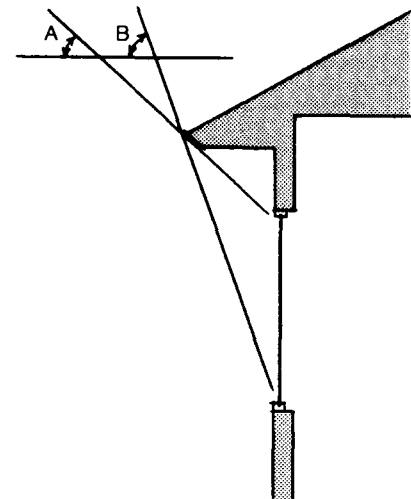
South Overhang Sizing In Indianapolis, an ideally sized south overhang should allow full exposure of the window when the sun has a noon altitude of 31 degrees (angle A) and fully shade the window when the sun has a noon altitude of 68 degrees (angle B).
