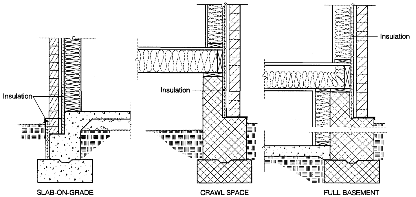
TYPES OF FOUNDATIONS
