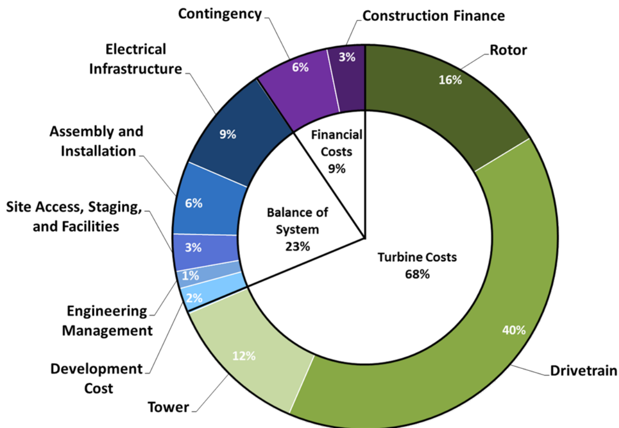
Figure 4. Capital expenditures for the land-based wind reference project
