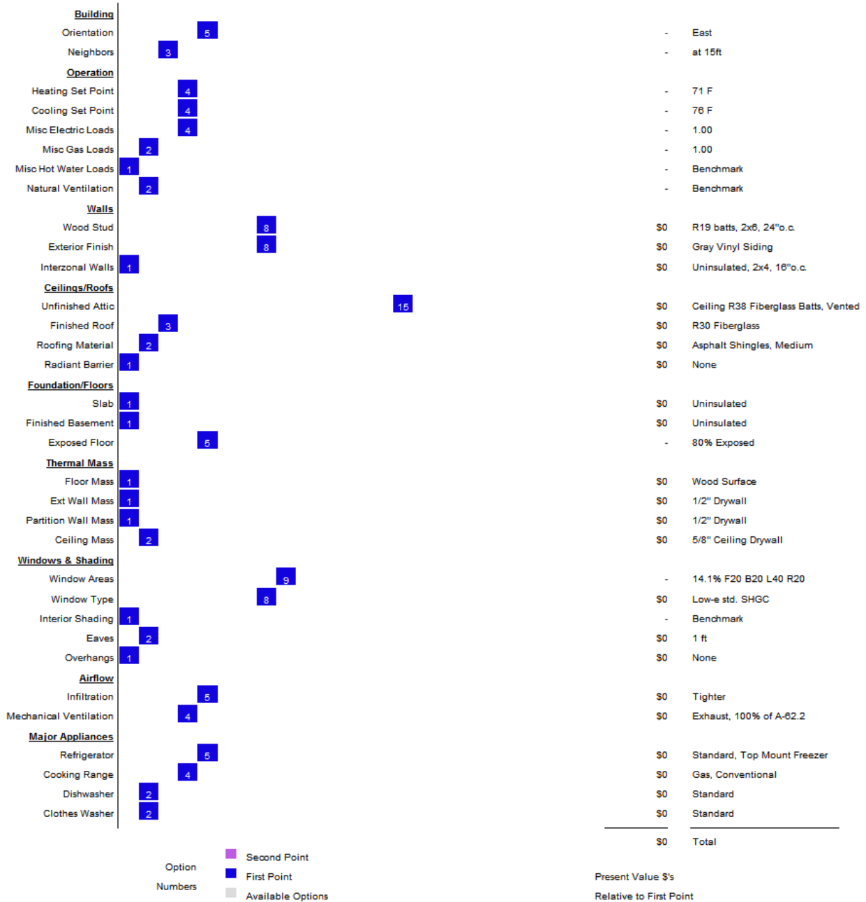
Figure 19. Full basement BEopt model house specification
