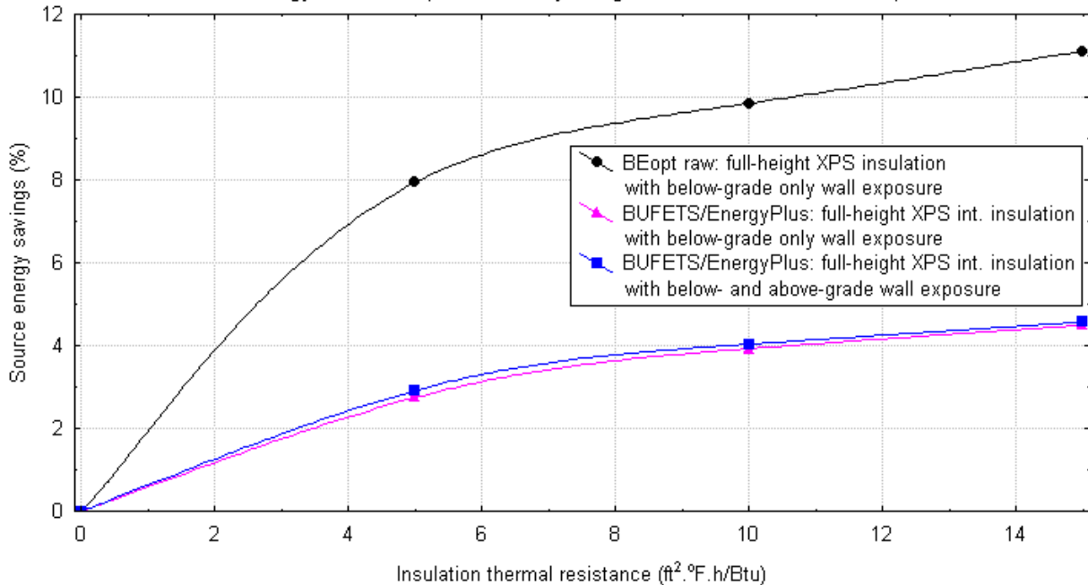
Figure 46. Source energy savings from crawlspace wall insulation for Bemidji
