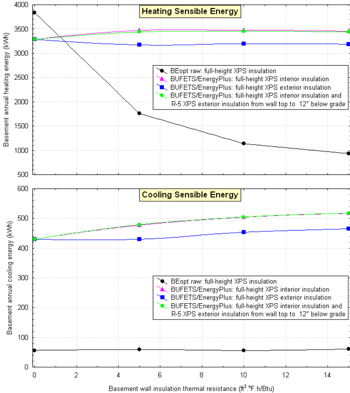
Figure 24. Absolute full basement energy consumption for Janesville
