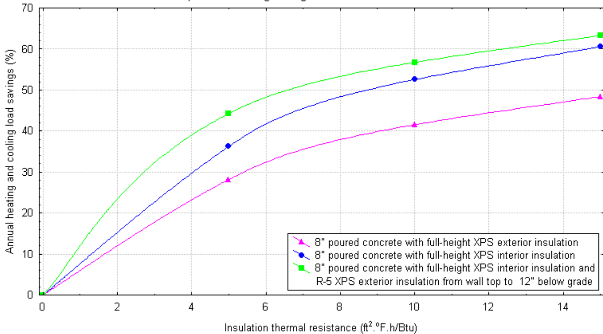
Figure 15. Annual full basement heating and cooling load energy savings for Janesville
