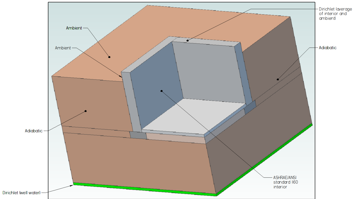
Figure 1. BUFETS boundary conditions
