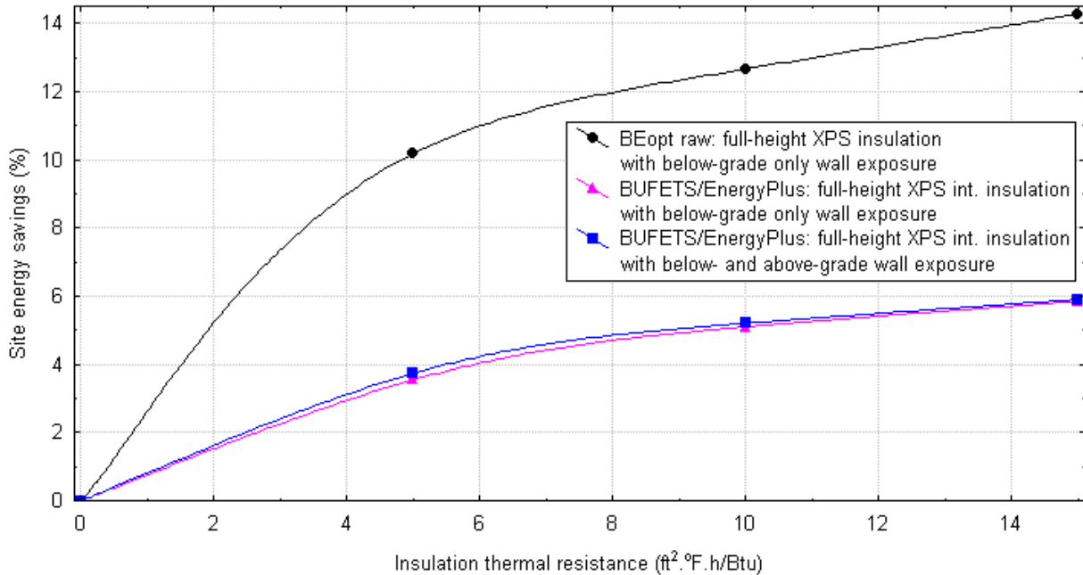
Figure 45. Site energy savings from crawlspace wall insulation for Bemidji
