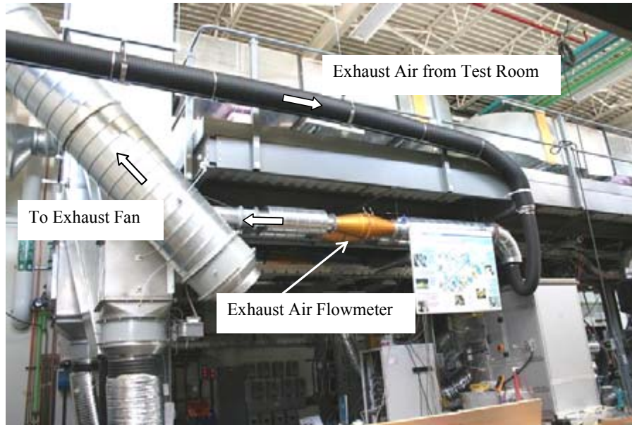
Figure 6. Exhaust system
