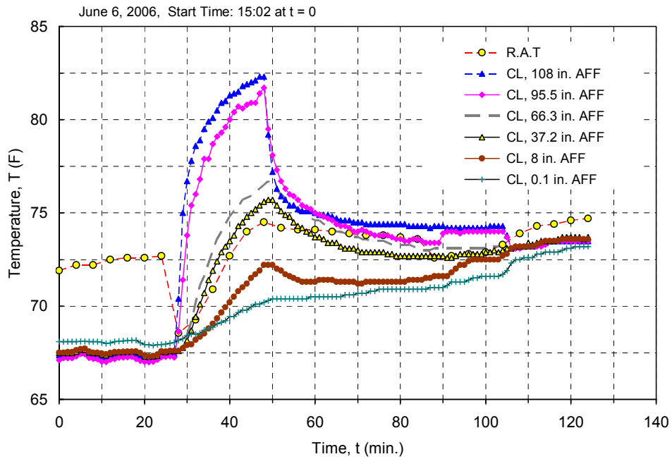
Figure 14. Centerline temperatures
