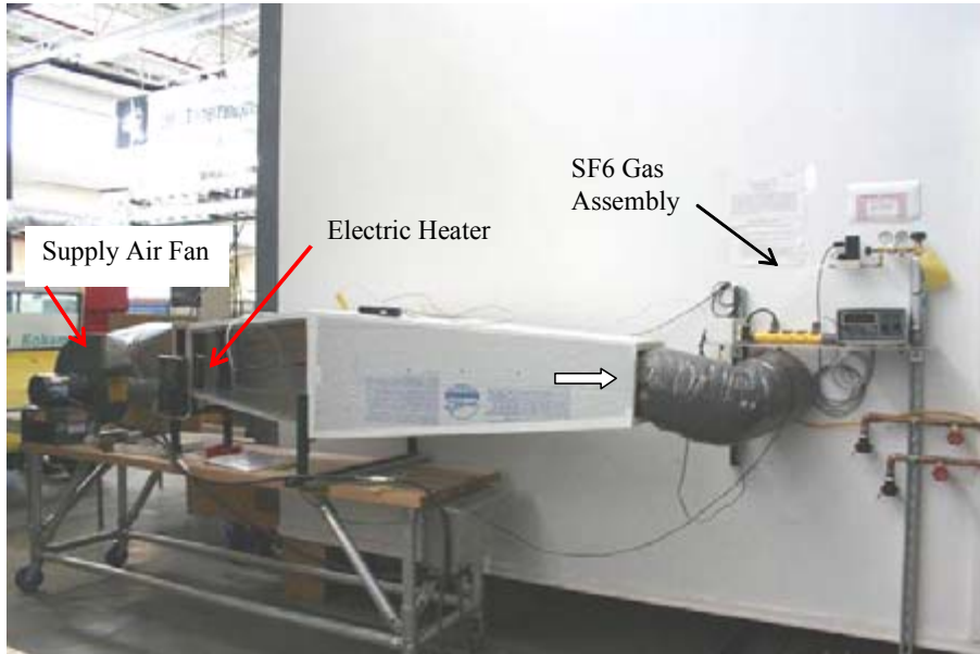
Figure 4. Supply-air apparatus
