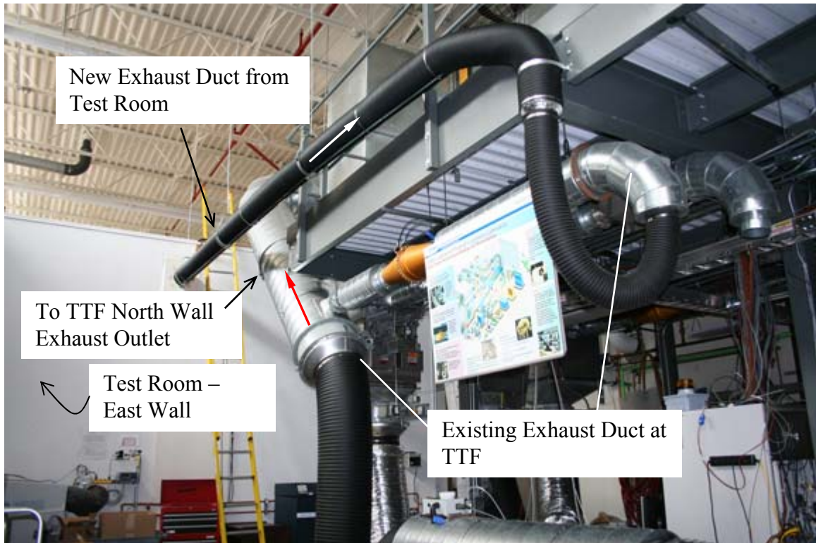
Figure 4. Exhaust Duct System of Thermal Conversion Laboratory at TTF
