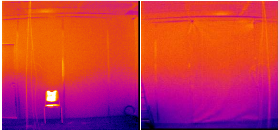
Figure 10. IR images of north and south walls
