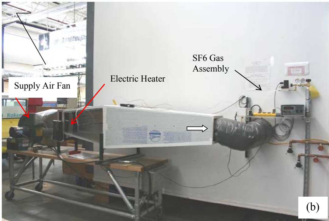
Figure 3. Schematic (a) and Photo (b) of Supply Air Apparatus – Not To Scale
