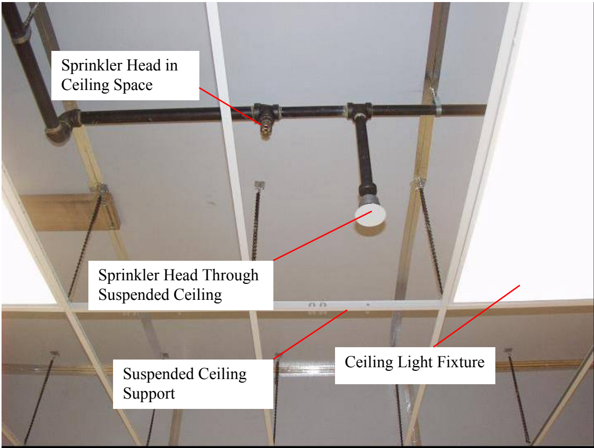
Figure 5. Existing Sprinkler System in Test Room
