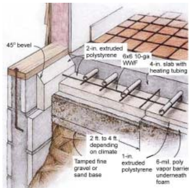
Radiant slab
