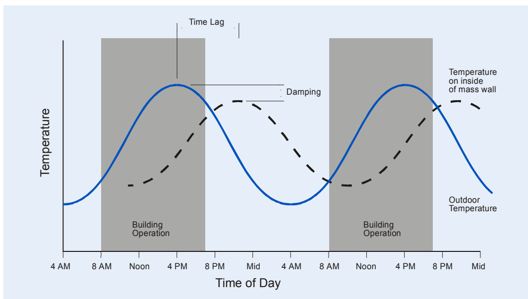
Figure 11 – Temperature Swing
