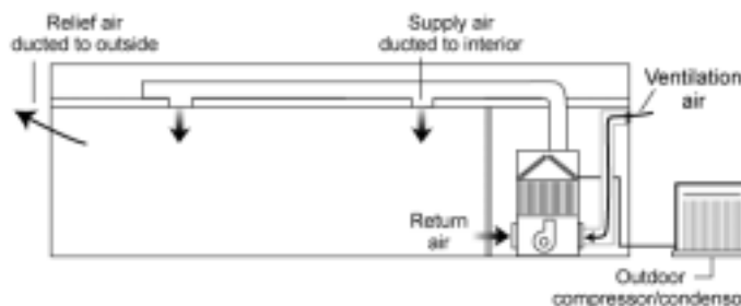
Basic gas/electric split system.
