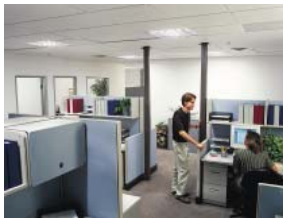
Tubular skylights in interior administrative office provide high lighting levels even when electric lights are off. Skylight diffuser panel fits into a standard suspended ceiling system.
