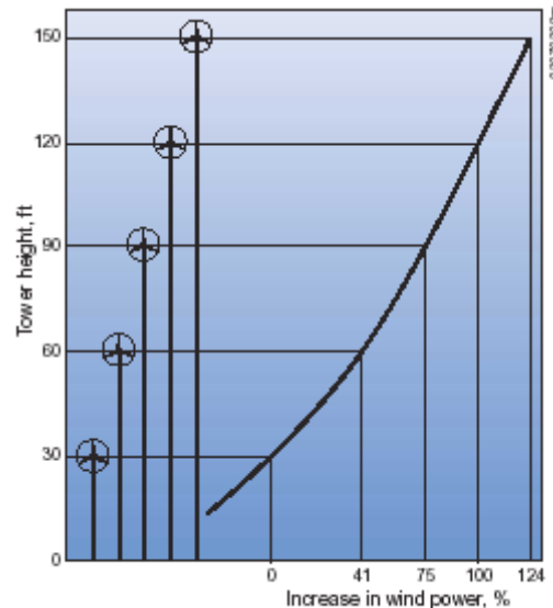
Figure 41 – Wind Speeds Increase with Height
