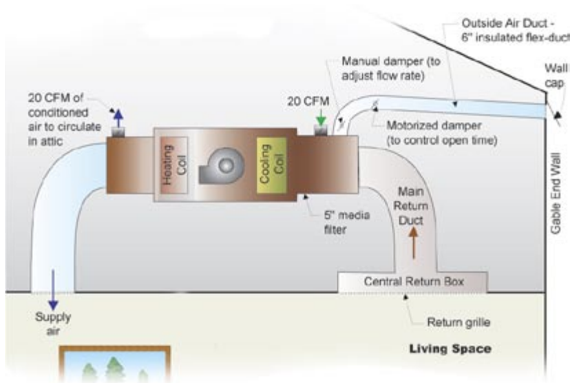
FIGURE 15: Outside Vents
