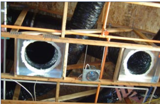
Careful duct sealing with mastic helps improve comfort and energy efficiency at low cost.
