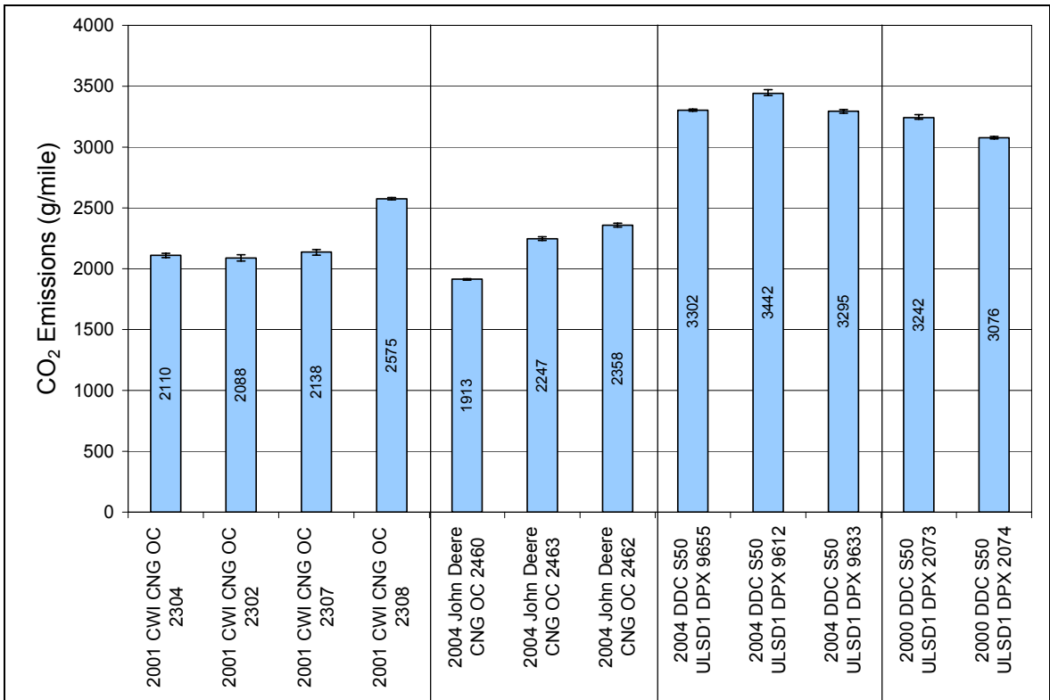
Figure 15: CO 2 Emissions
