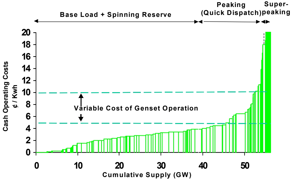
Figure 4-3. On-site generation
