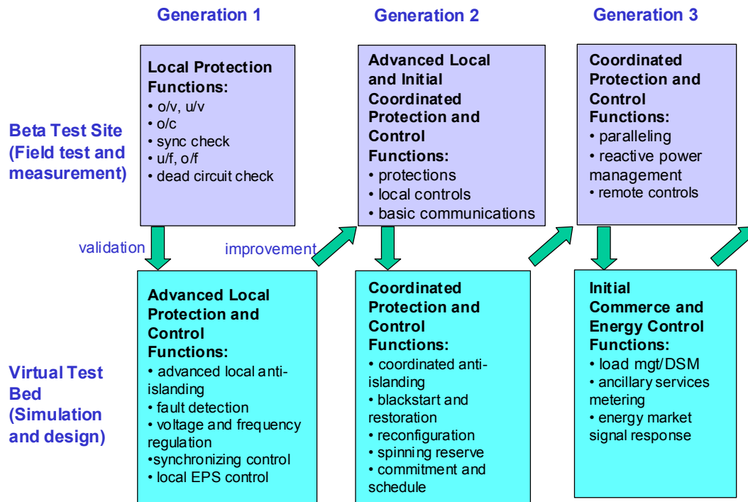
Figure 3-9. Interconnect technology roadmap
