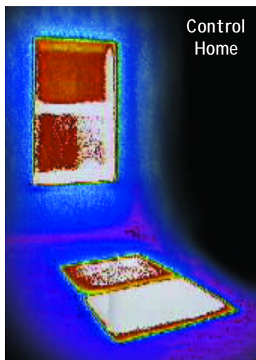
Comparison of the infrared appearance of west-facing windows of both homes in the afternoon. The Zero Energy home's windows accounted for almost one-fifth of the energy savings (for cooling).
