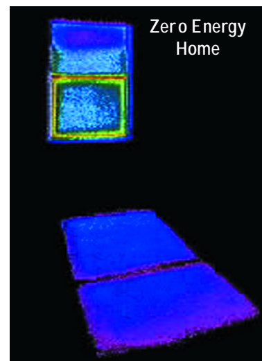
Comparison of the infrared appearance of west-facing windows of both homes in the afternoon. The Zero Energy home's windows accounted for almost one-fifth of the energy savings (for cooling).
