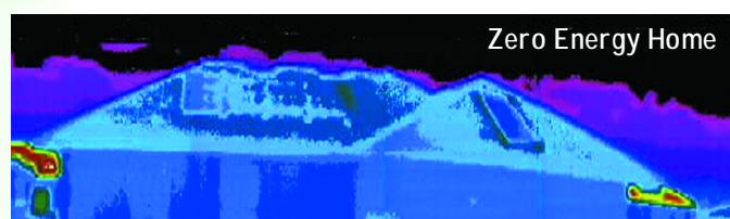
Thermographic images of the roofs in both homes. Note the lower roof and attic heat gain into the Zero Energy home, thus reducing the demand for cooling.
