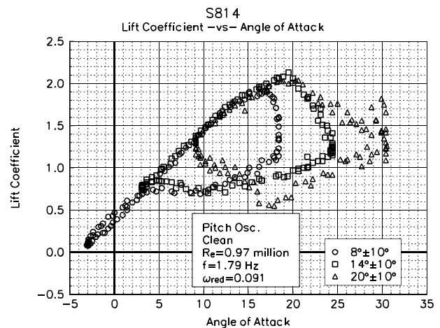
Figure 29. Clean, C_l vs \alpha , \omega_{red}=0.091 , \pm 10^\circ
