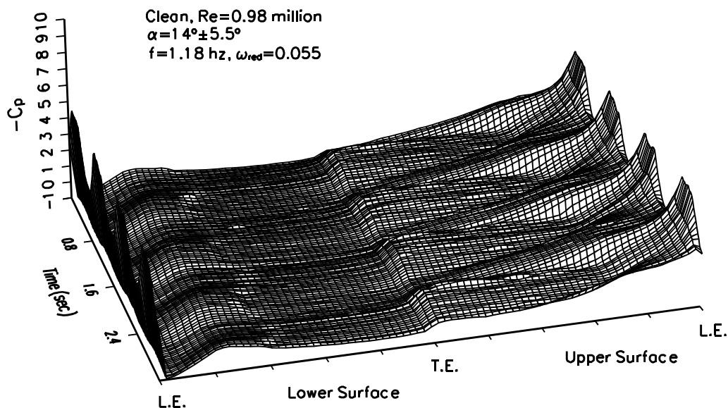
Figure 36. Unsteady pressure distribution, clean, \omega_{red}=0.055 , 14 \pm 5.5^\circ
