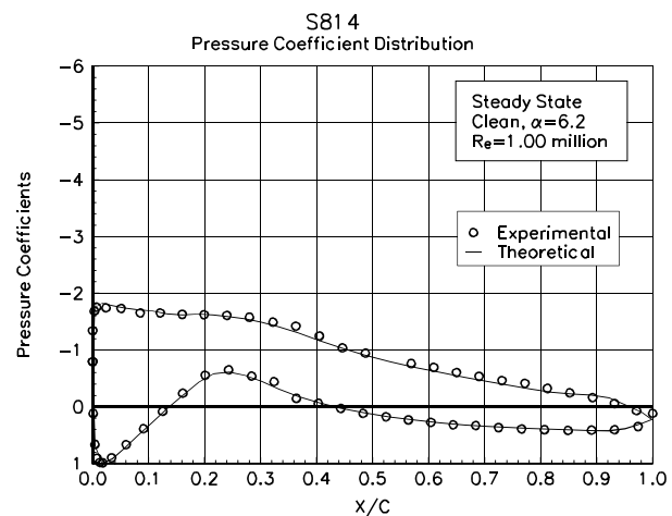
Figure 11. Comparison with theory, C_p vs x/c , \alpha=6.2^\circ
