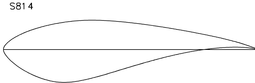
Figure 4. S814 airfoil section
