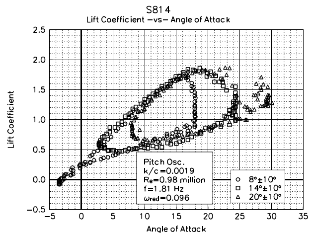
Figure 33. LEGR, C_l vs \alpha , \omega_{red}=0.096 , \pm 10^\circ
