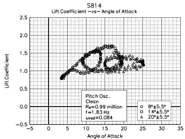
Figure 21. Clean, C_l vs \alpha , \omega_{red}=0.084 , \pm 5.5^\circ
