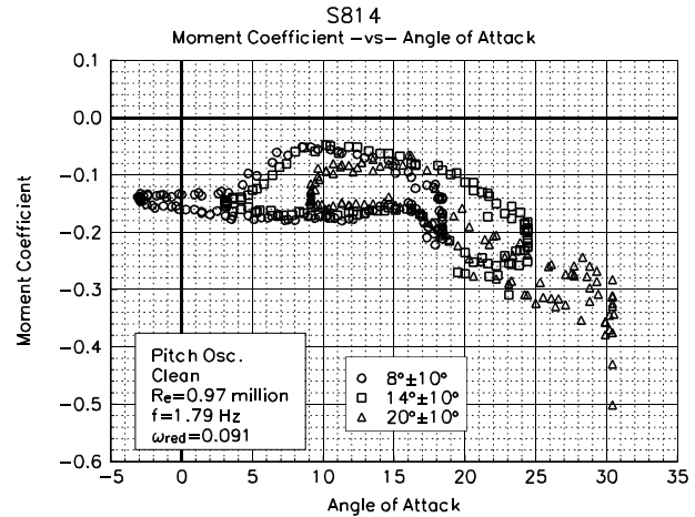
Figure 31. Clean, C_m vs \alpha , \omega_{red}=0.091 , \pm 10^\circ
