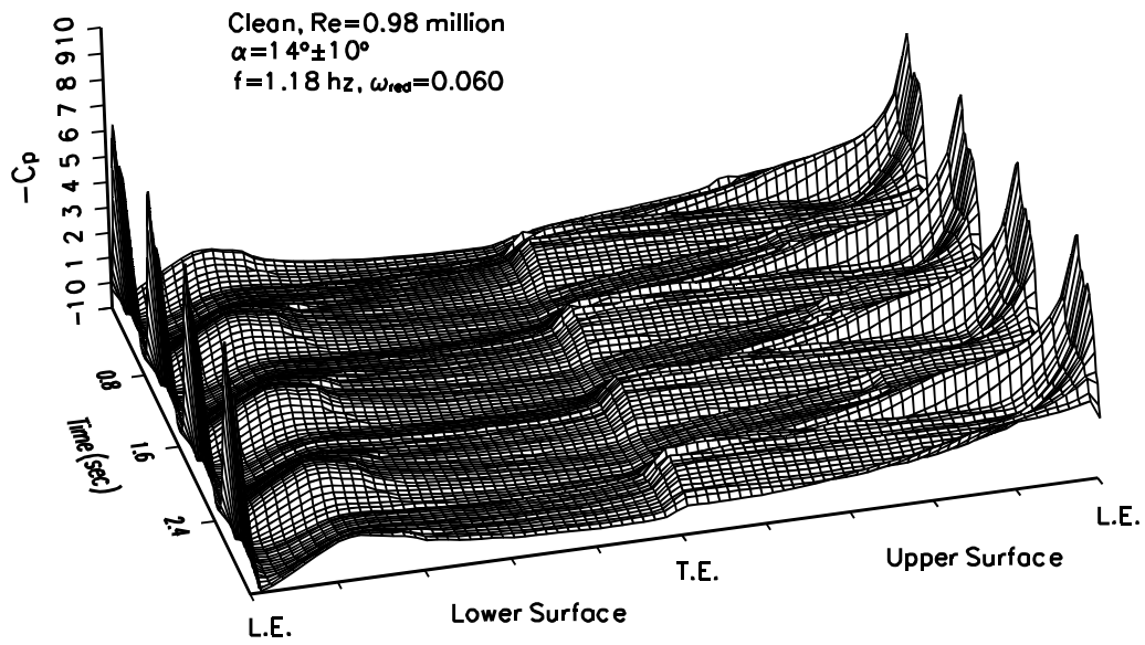
Figure 38. Unsteady pressure distribution, clean, \omega_{red}=0.060 , 14^\circ \pm 10^\circ
