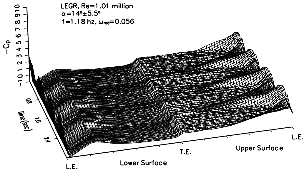
Figure 37. Unsteady pressure distribution, LEGR, \omega_{red}=0.056 , 14 \pm 5.5^\circ
