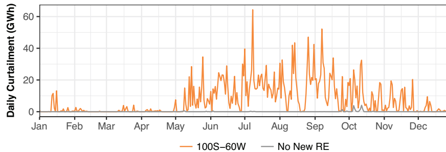
Total daily curtailment throughout the year in Tamil Nadu
