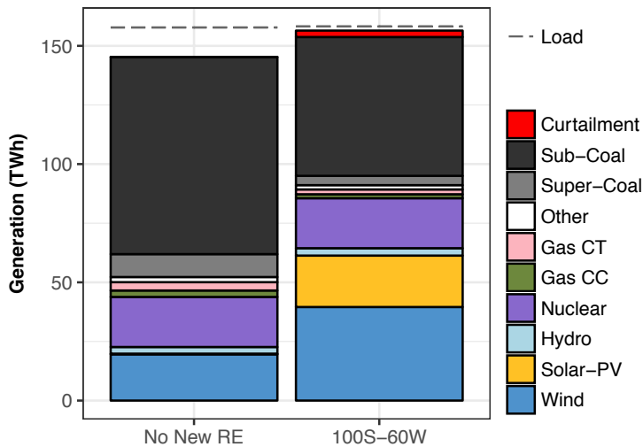
Annual energy generation in Tamil Nadu
