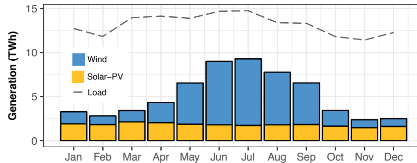
RE penetration by load and generation
