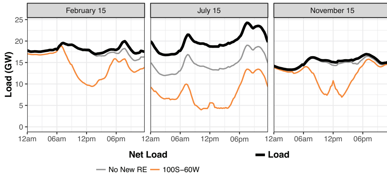
Example days of load and net load in Tamil Nadu
