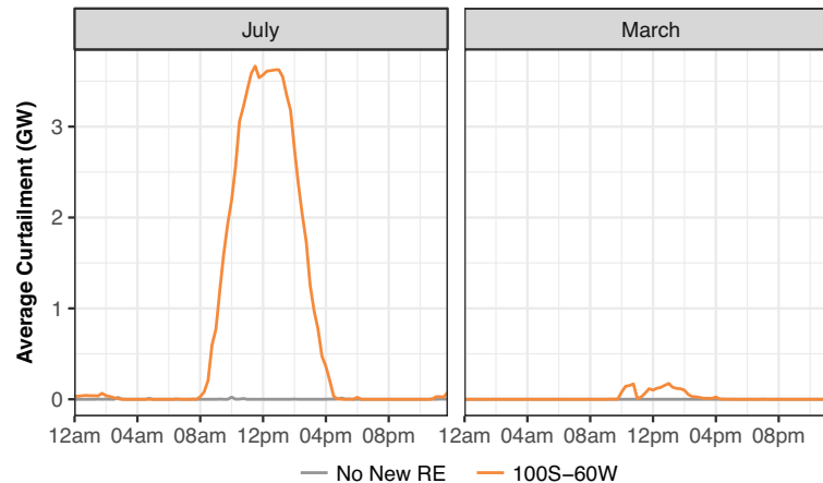
Average daily curtailment in March and July in Tamil Nadu
