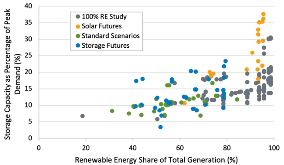
Figure 11. Storage capacity as a function of renewable energy contribution (%).
